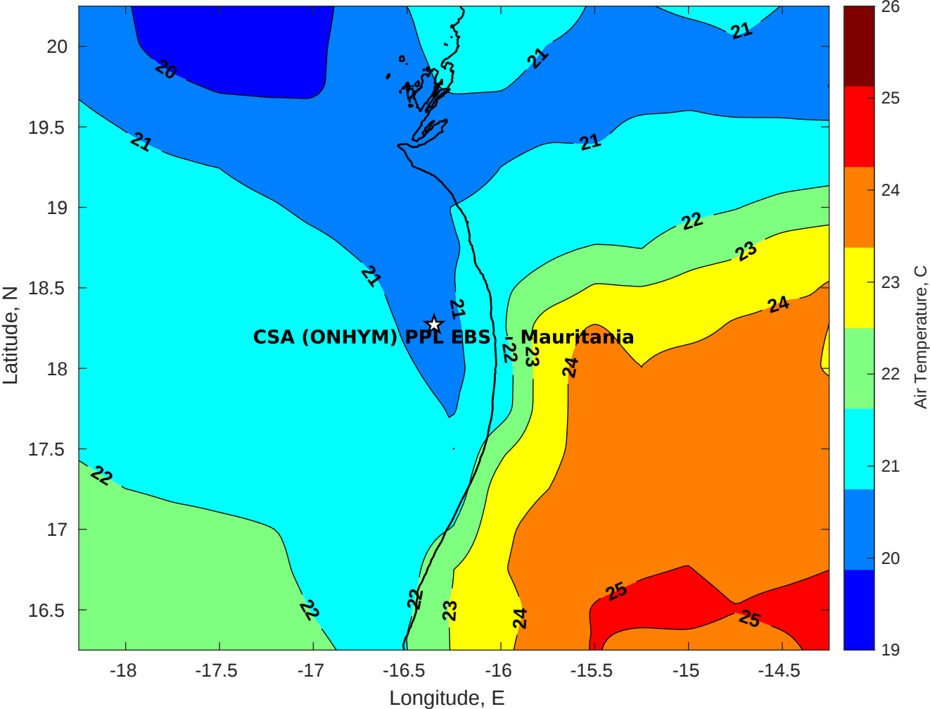
Air Temperature (C) for CSA (ONHYM) PPL EBS - Mauritania at 28-Dec-2025
