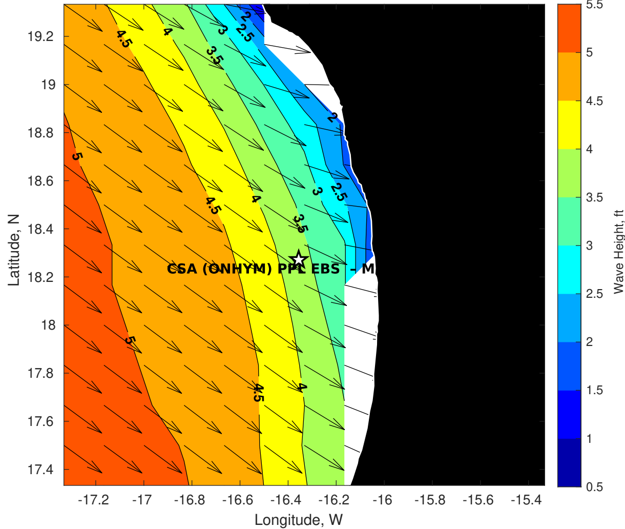
GFS Wave Height (ft) for CSA (ONHYM) PPL EBS - Mauritania at 28-Dec-2025 09:00:00
