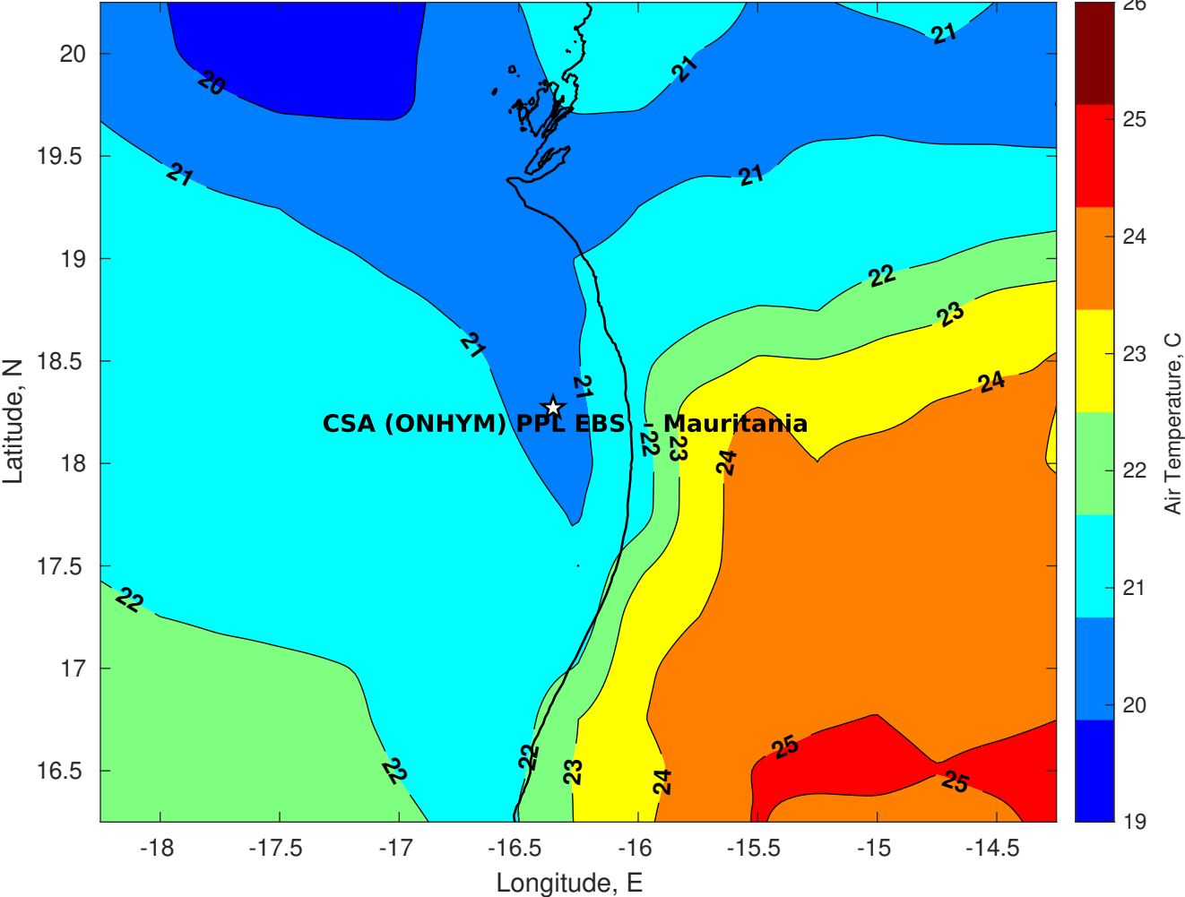
Air Temperature (C) for CSA (ONHYM) PPL EBS - Mauritania at 28-Dec-2025
