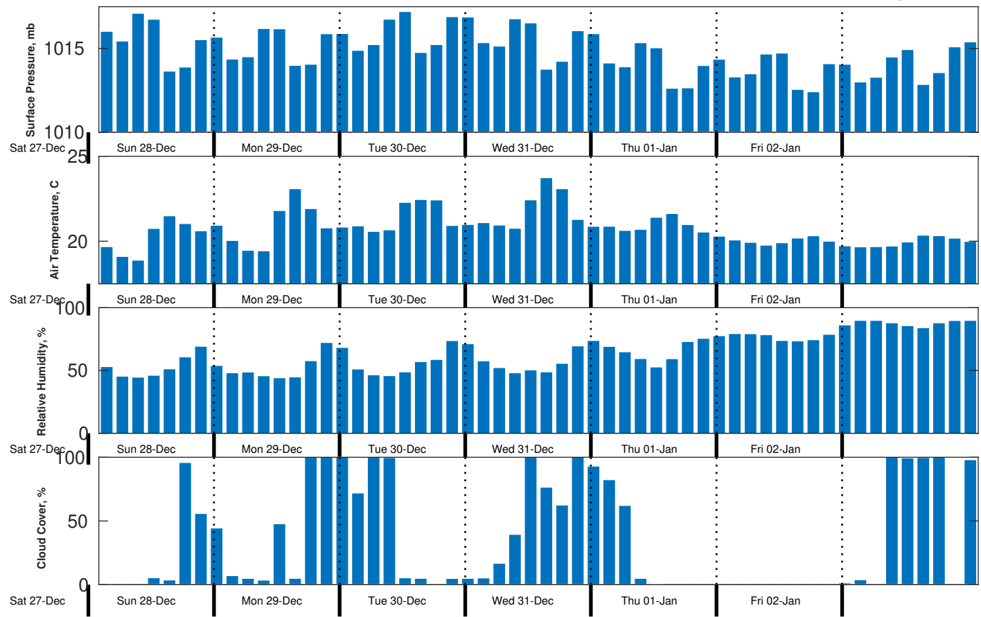
Met Forecast for CSA (ONHYM) PPL EBS - Mauritania from 28-Dec-2025 00:00:00 to 04-Jan-2026 00:00:00
