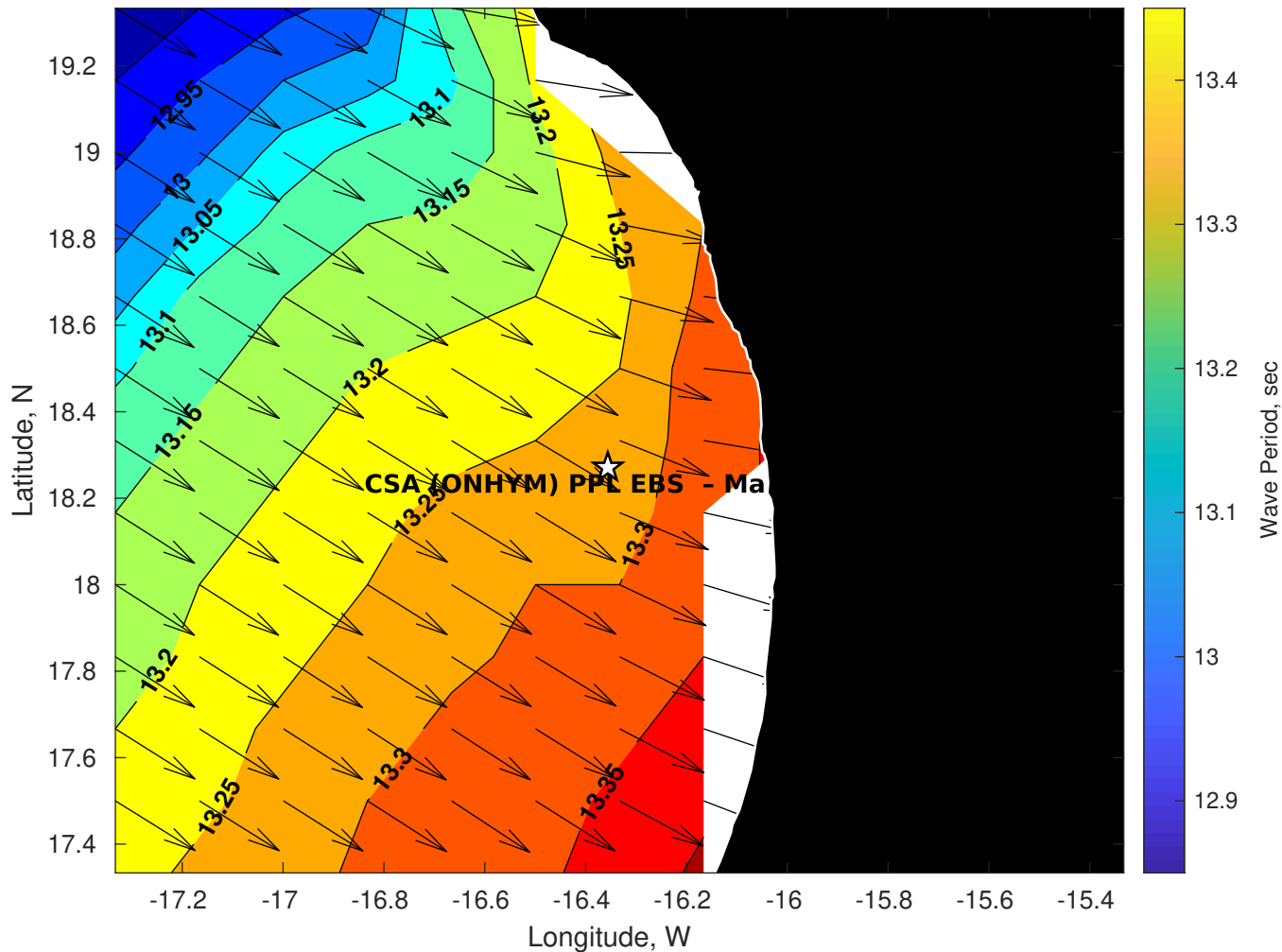
GFS Wave Period (sec) for CSA (ONHYM) PPL EBS - Mauritania at 28-Dec-2025 09:00:00
