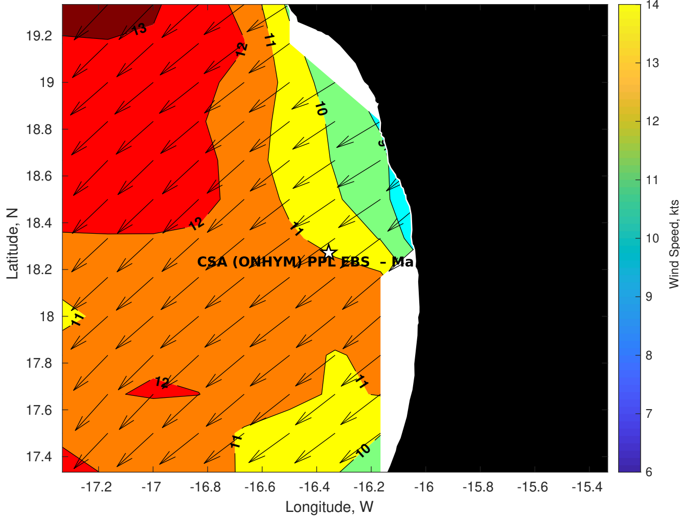
GFS Winds (kts) for CSA (ONHYM) PPL EBS - Mauritania at 28-Dec-2025 09:00:00
