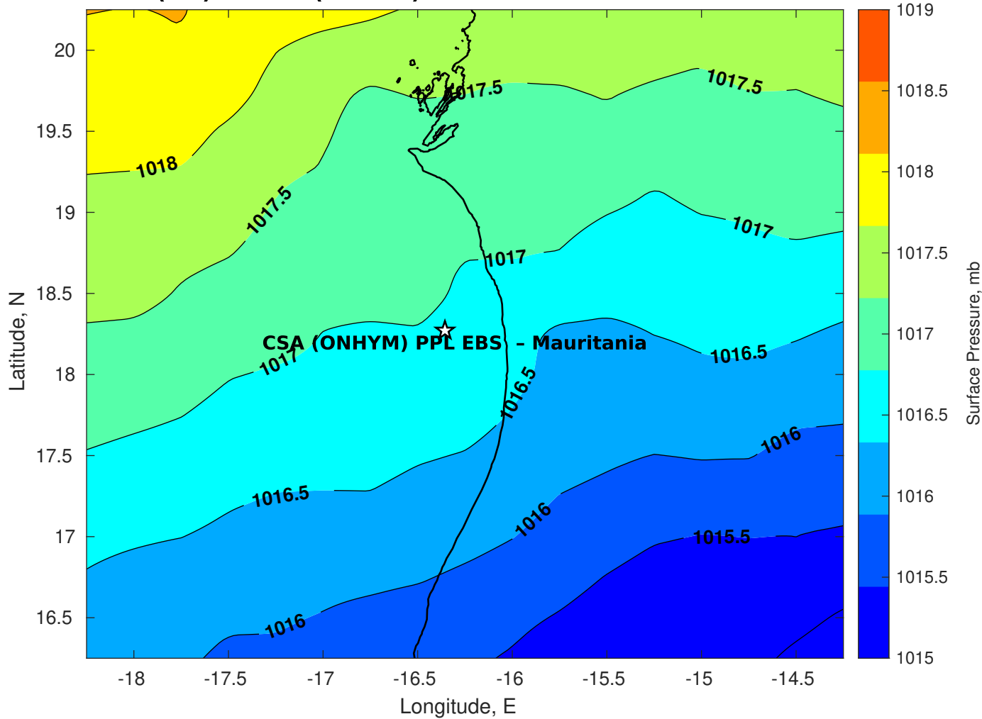
Surface Pressure (mb) for CSA (ONHYM) PPL EBS - Mauritania at 28-Dec-2025 00:00:00
