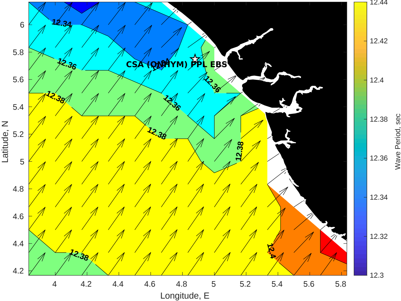
GFS Wave Period (sec) for CSA (ONHYM) PPL EBS - Nigeria at 28-Dec-2025 09:00:00
