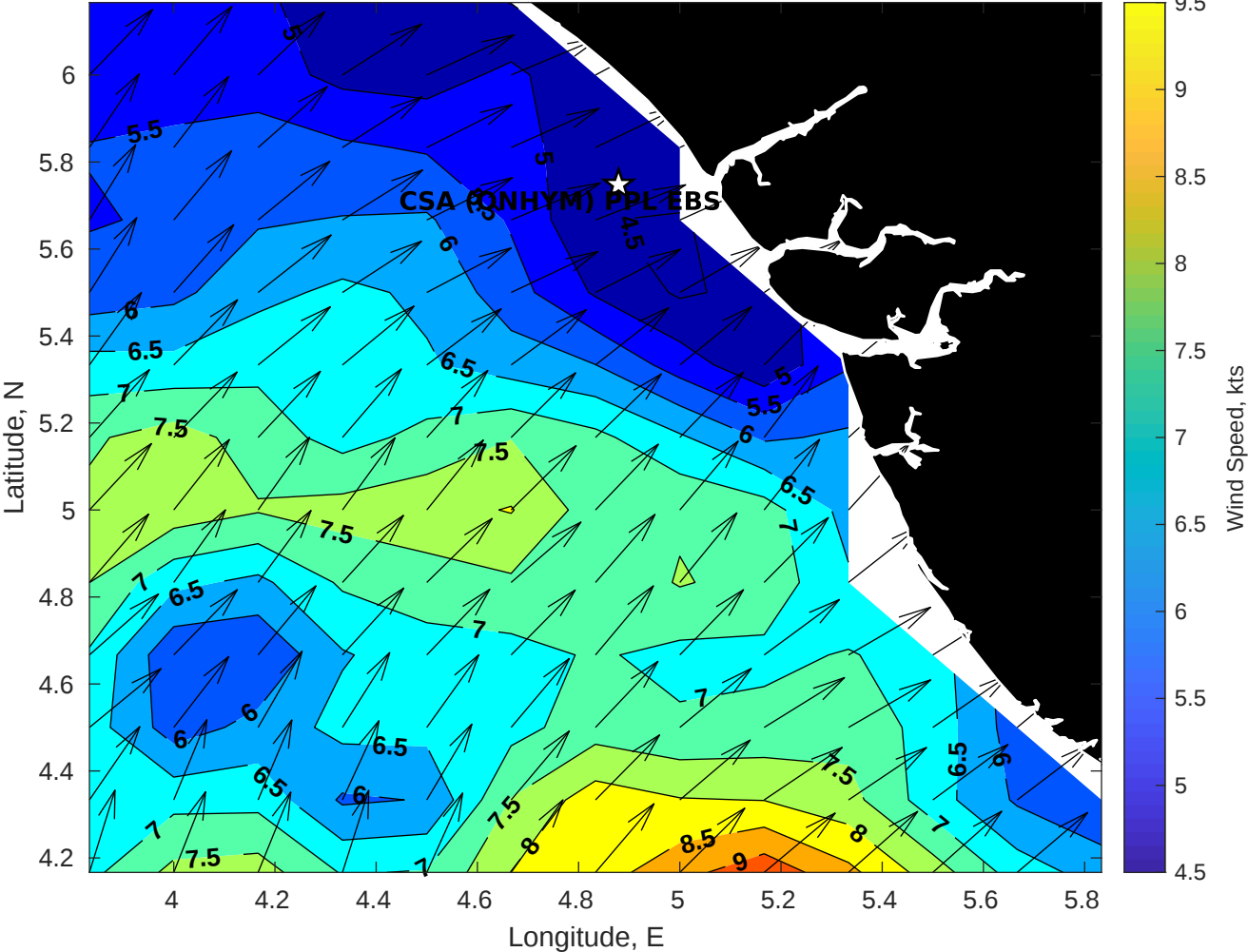
GFS Winds (kts) for CSA (ONHYM) PPL EBS - Nigeria at 28-Dec-2025 09:00:00
