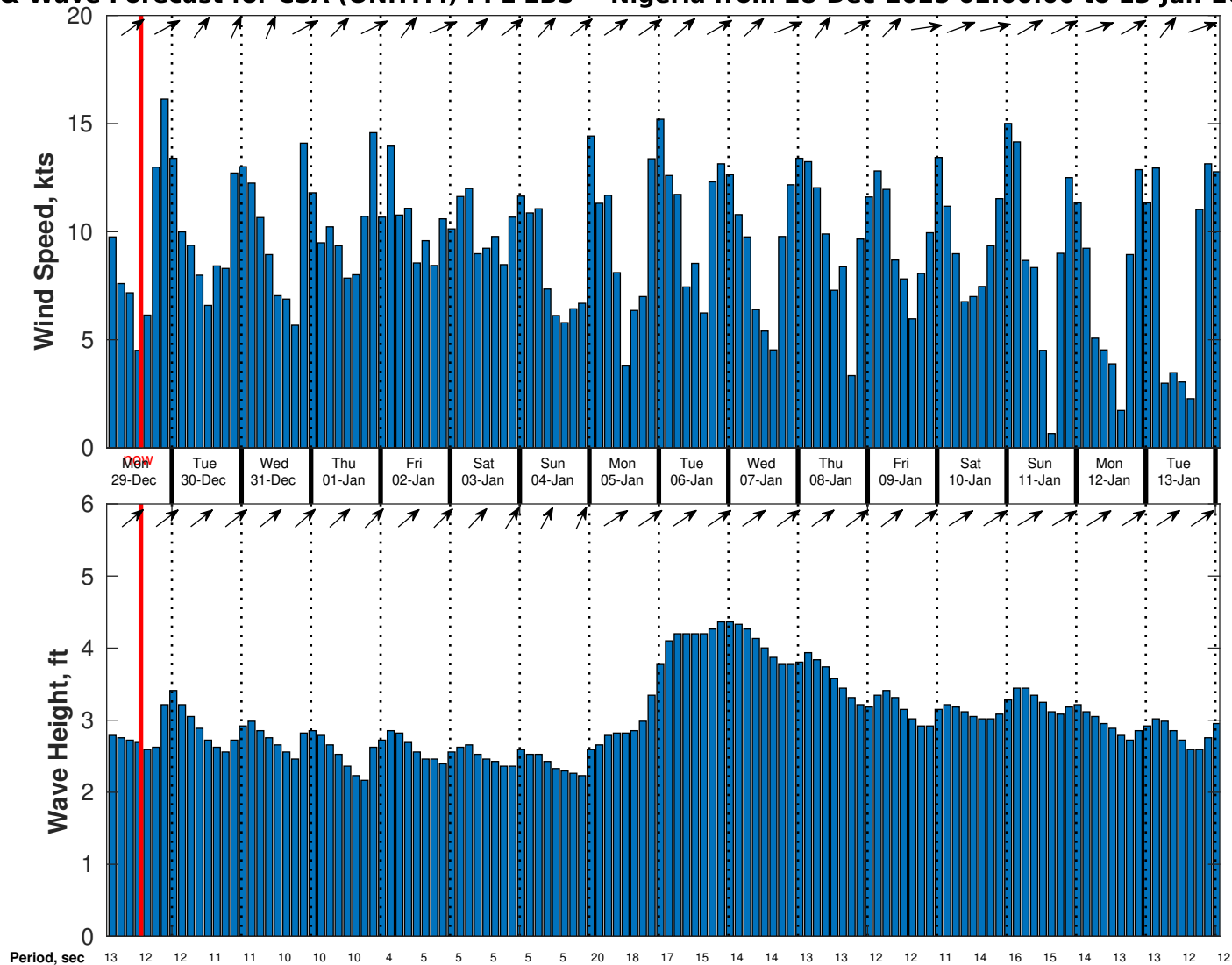
Wind & Wave Forecast for CSA (ONHYM) PPL EBS - Nigeria from 28-Dec-2025 02:00:00 to 13-Jan-2026 02:00:00
