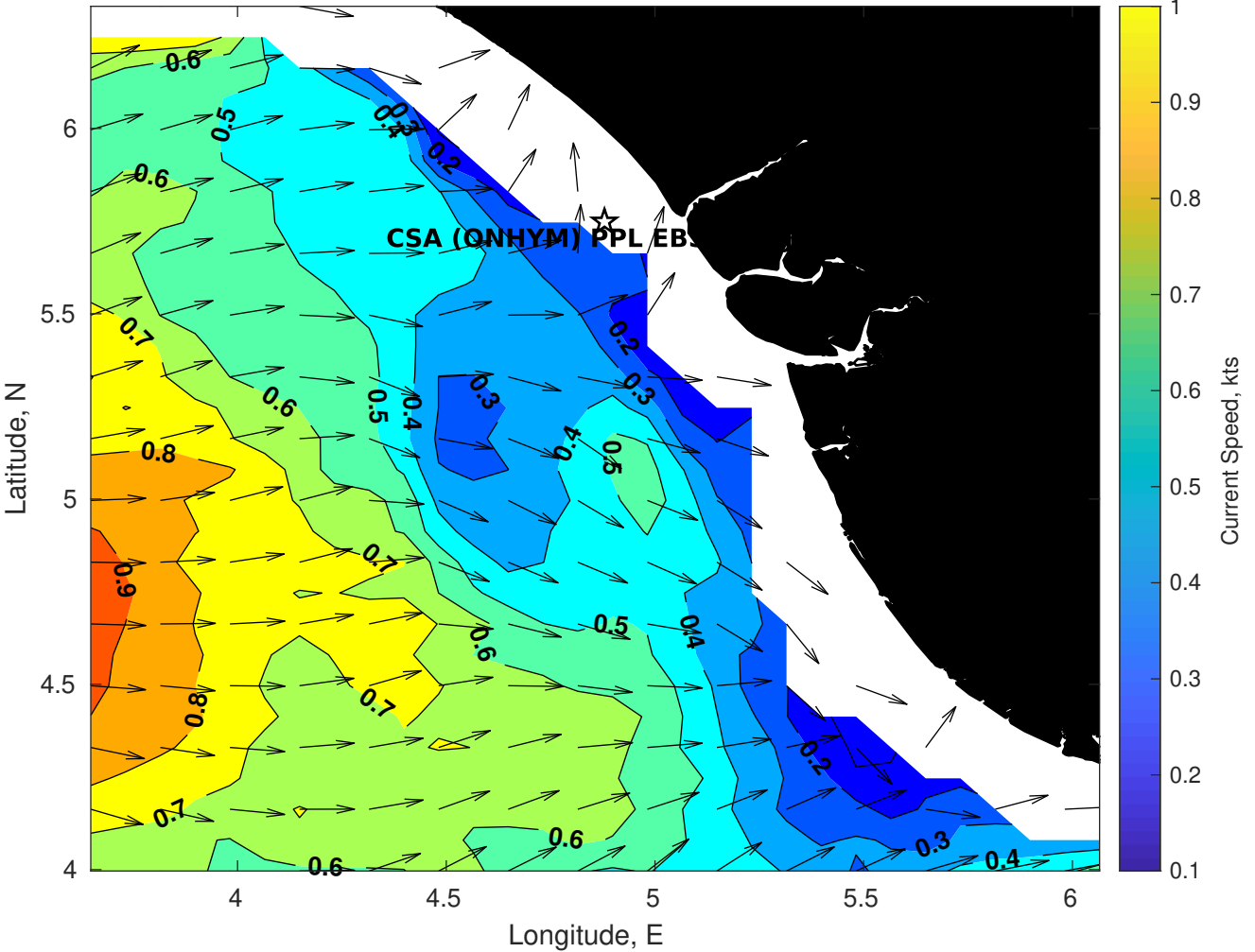
Surface Currents for CSA (ONHYM) PPL EBS - Nigeria at 27-Dec-2025 00:00:00
