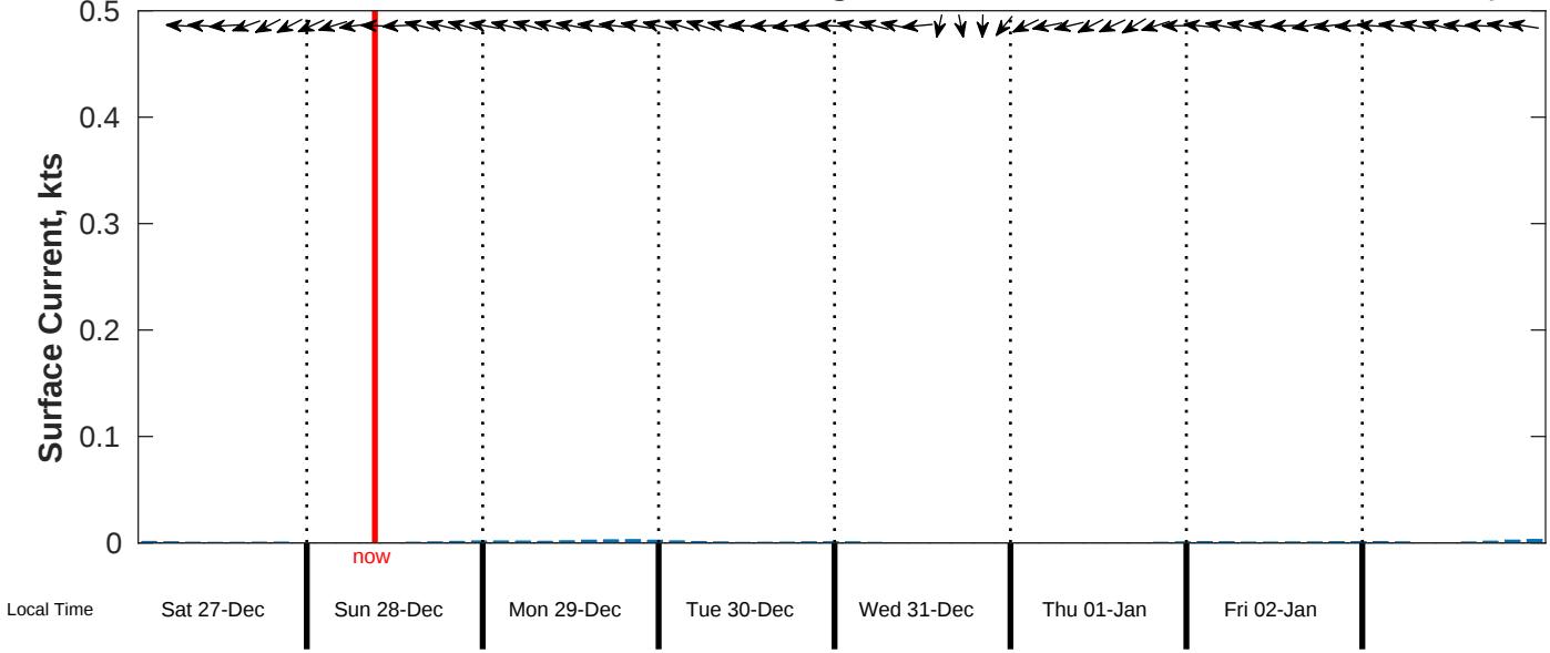
Surface Current Forecast for CSA (ONHYM) PPL EBS - Nigeria from 27-Dec-2025 00:00:00 to 04-Jan-2026 00:00:00
