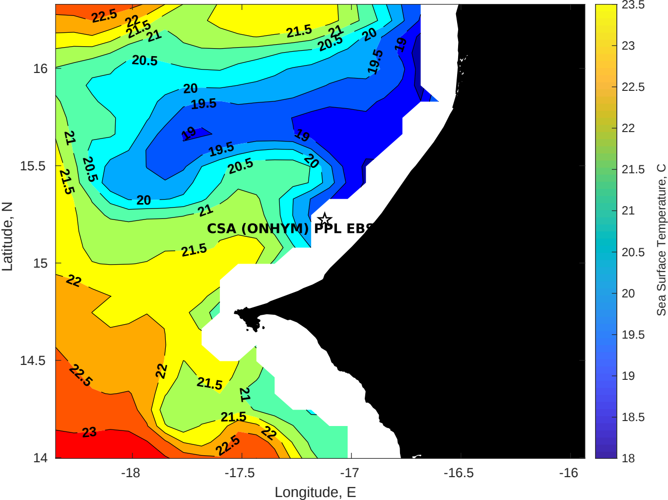
SST for CSA (ONHYM) PPL EBS - Senegal at 27-Dec-2025 00:00:00
