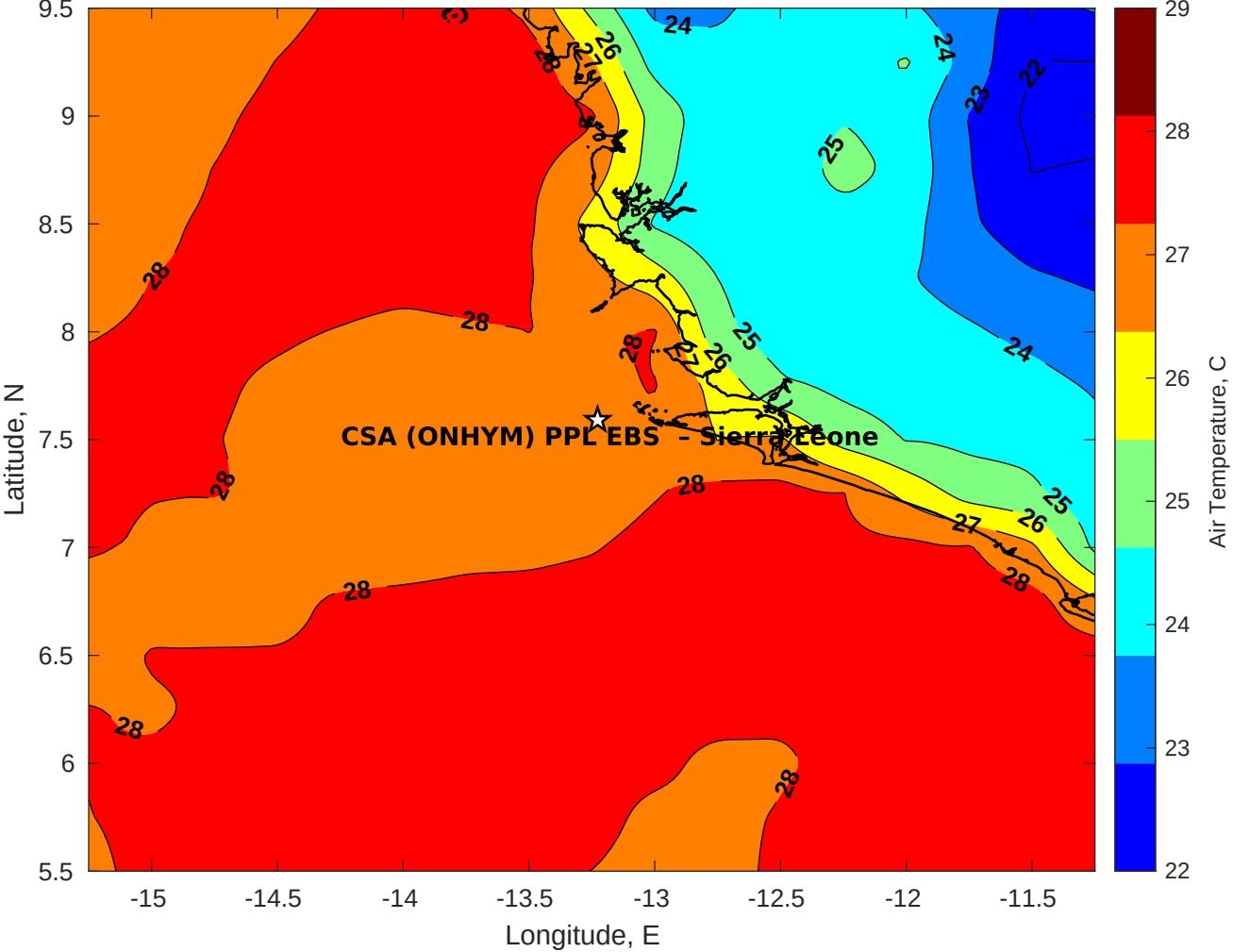
Air Temperature (C) for CSA (ONHYM) PPL EBS - Sierra Leone at 28-Dec-2025
