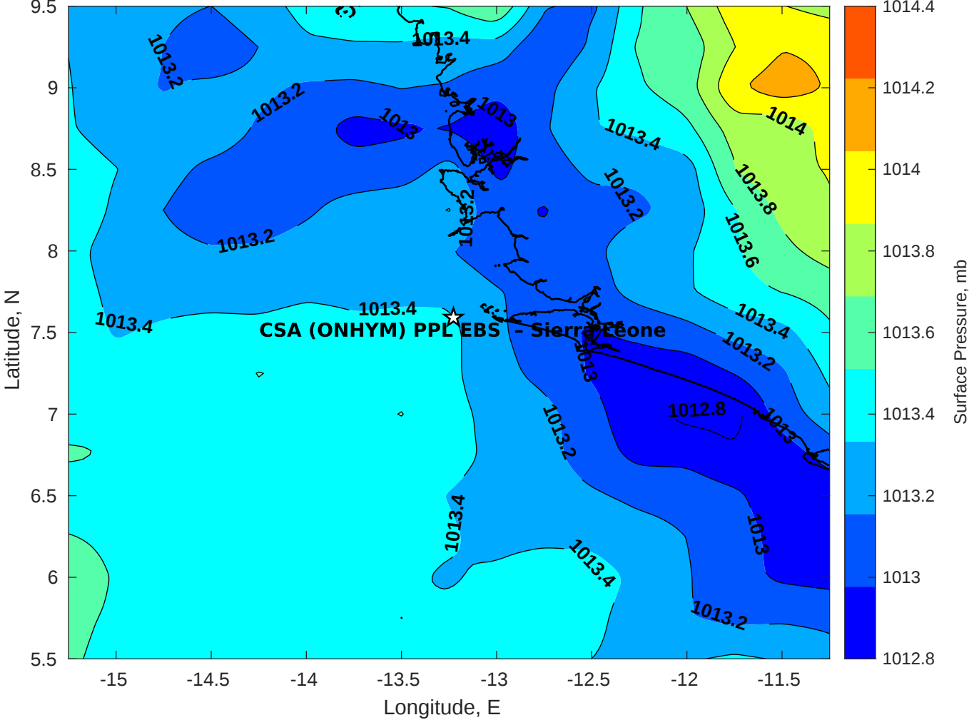
Surface Pressure (mb) for CSA (ONHYM) PPL EBS - Sierra Leone at 28-Dec-2025 00:00:00
