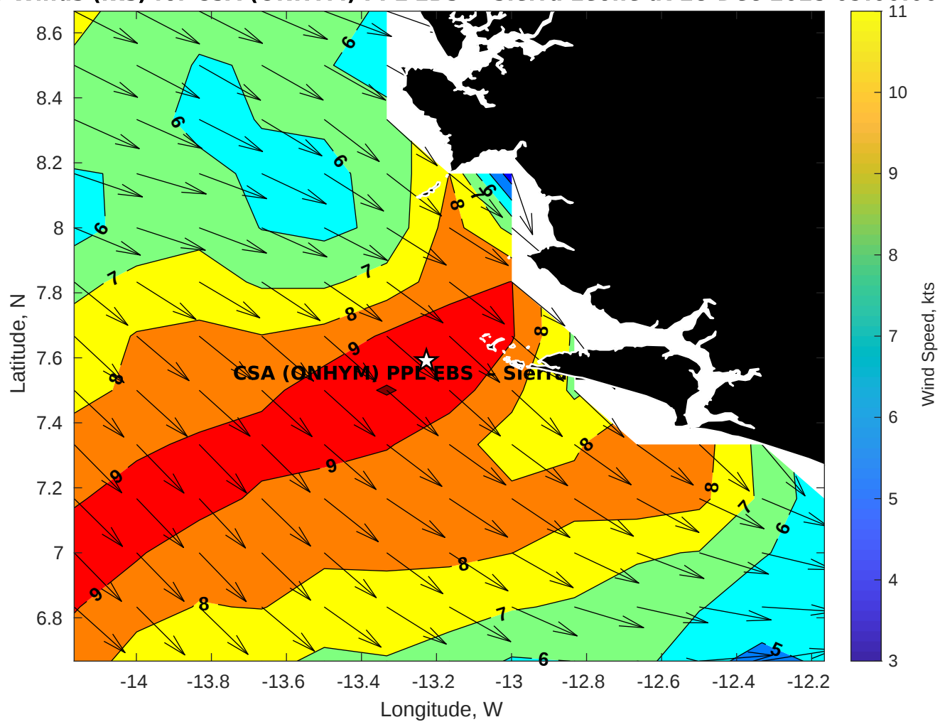
GFS Winds (kts) for CSA (ONHYM) PPL EBS - Sierra Leone at 28-Dec-2025 09:00:00
