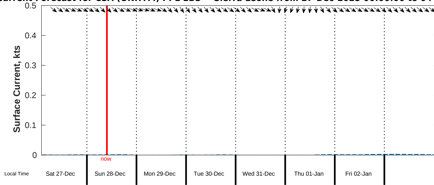
Surface Current Forecast for CSA (ONHYM) PPL EBS - Sierra Leone from 27-Dec-2025 00:00:00 to 04-Jan-2026 00:00:00
