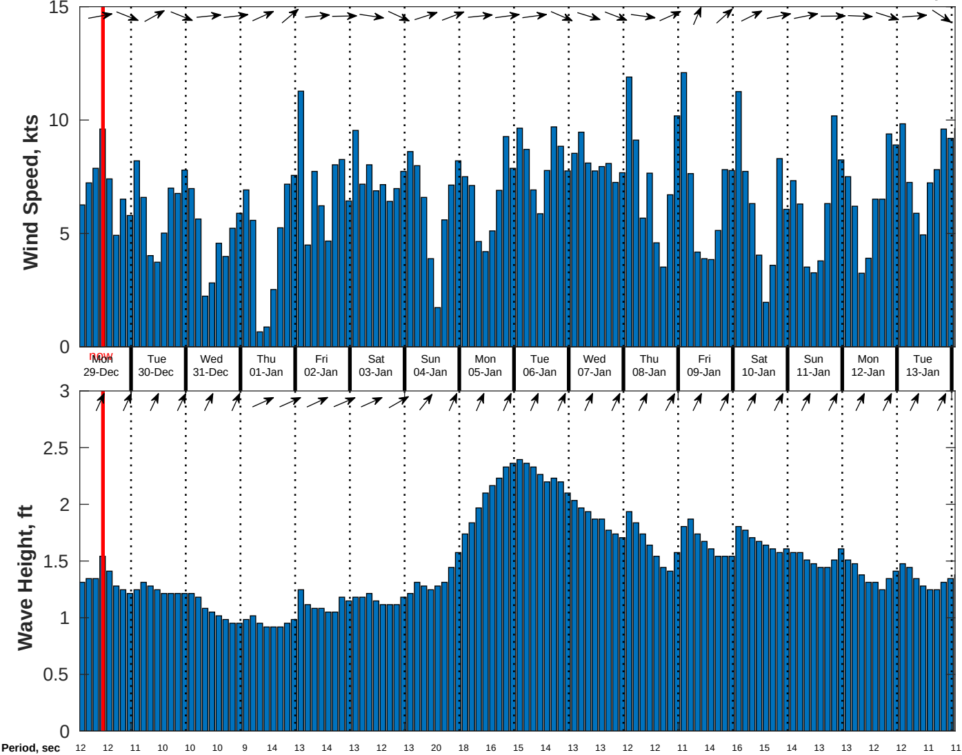
Wind & Wave Forecast for CSA (ONHYM) PPL EBS - Sierra Leone from 28-Dec-2025 01:00:00 to 13-Jan-2026 01:00:00
