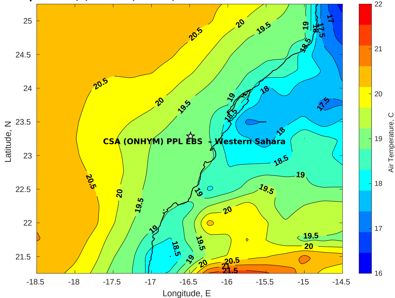
Air Temperature (C) for CSA (ONHYM) PPL EBS - Western Sahara at 28-Dec-2025
