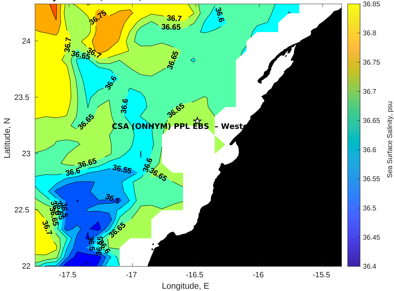
Surface Salinity for CSA (ONHYM) PPL EBS - Western Sahara at 27-Dec-2025 00:00:00
