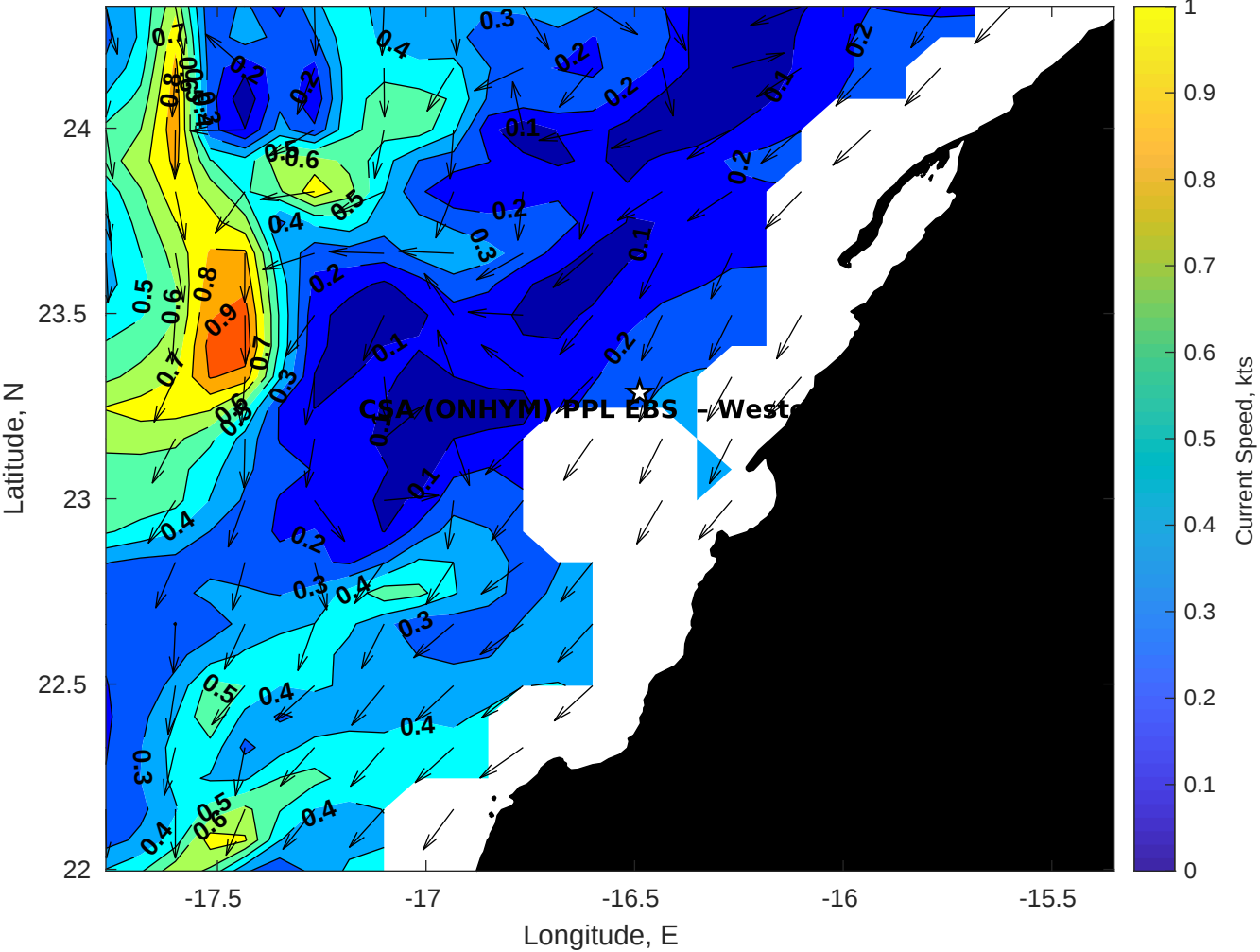
Surface Currents for CSA (ONHYM) PPL EBS - Western Sahara at 27-Dec-2025 00:00:00
