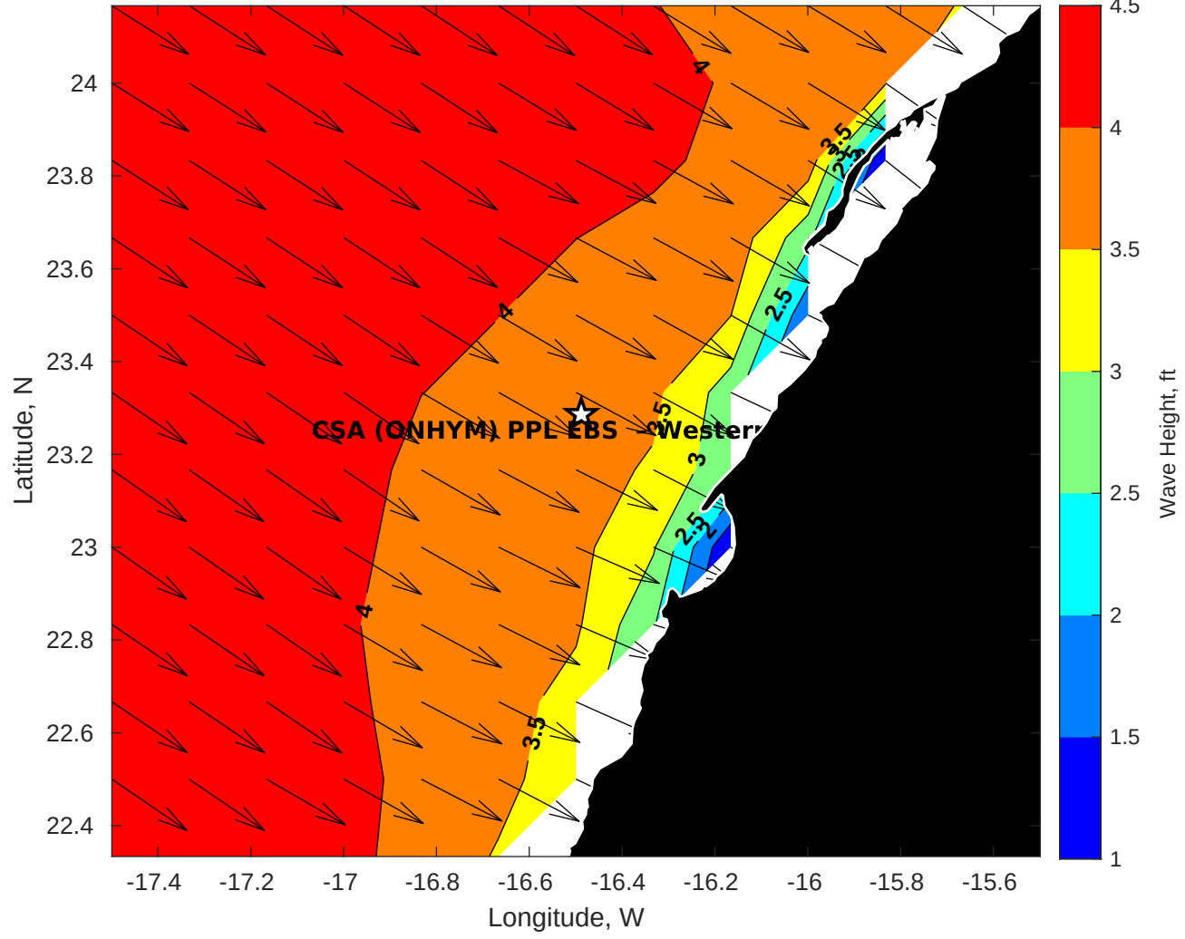
GFS Wave Height (ft) for CSA (ONHYM) PPL EBS - Western Sahara at 28-Dec-2025 09:00:00
