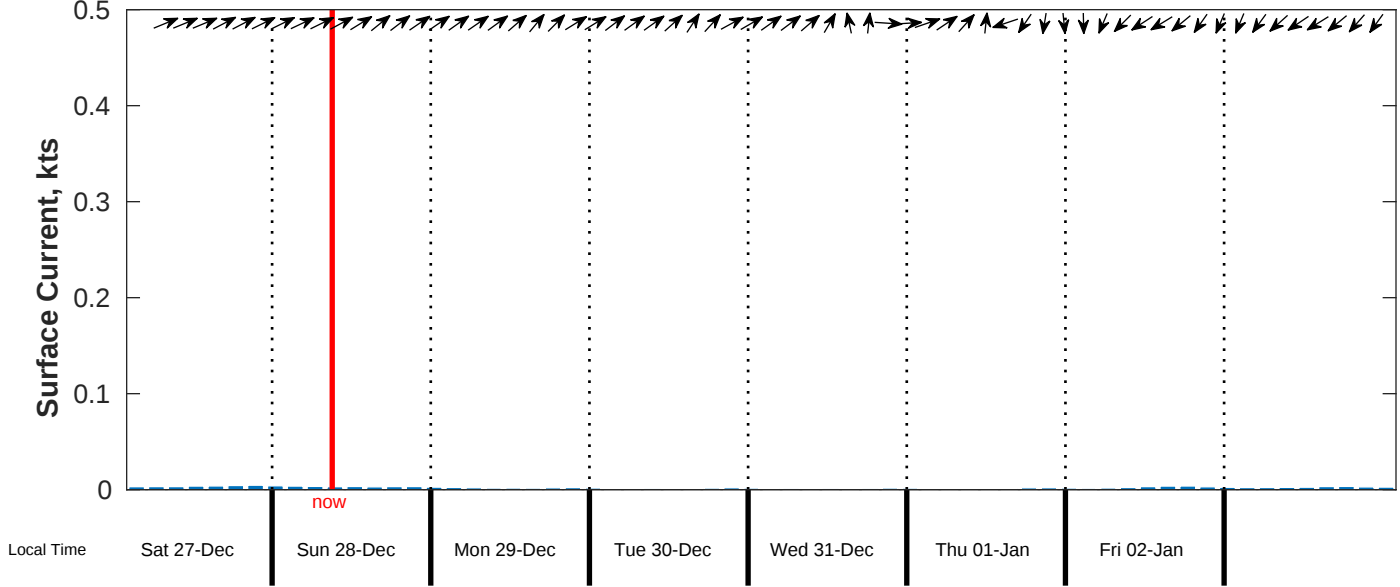
Surface Current Forecast for CSA (ONHYM) PPL EBS - Western Sahara from 27-Dec-2025 00:00:00 to 04-Jan-2026 00:00:00
