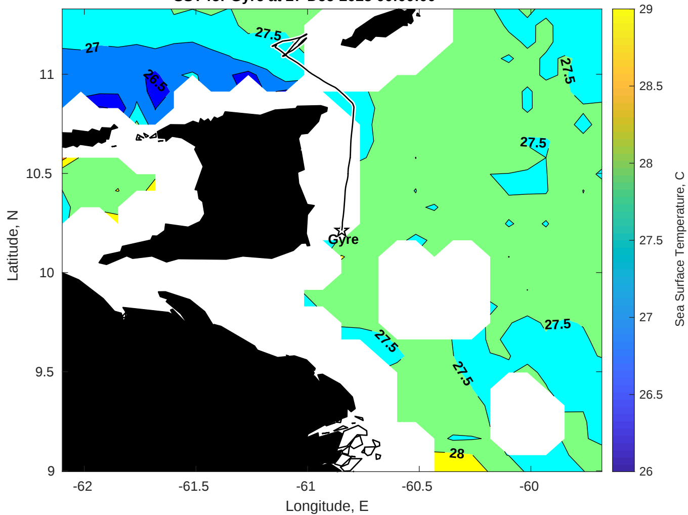
SST for Gyre at 27-Dec-2025 00:00:00
