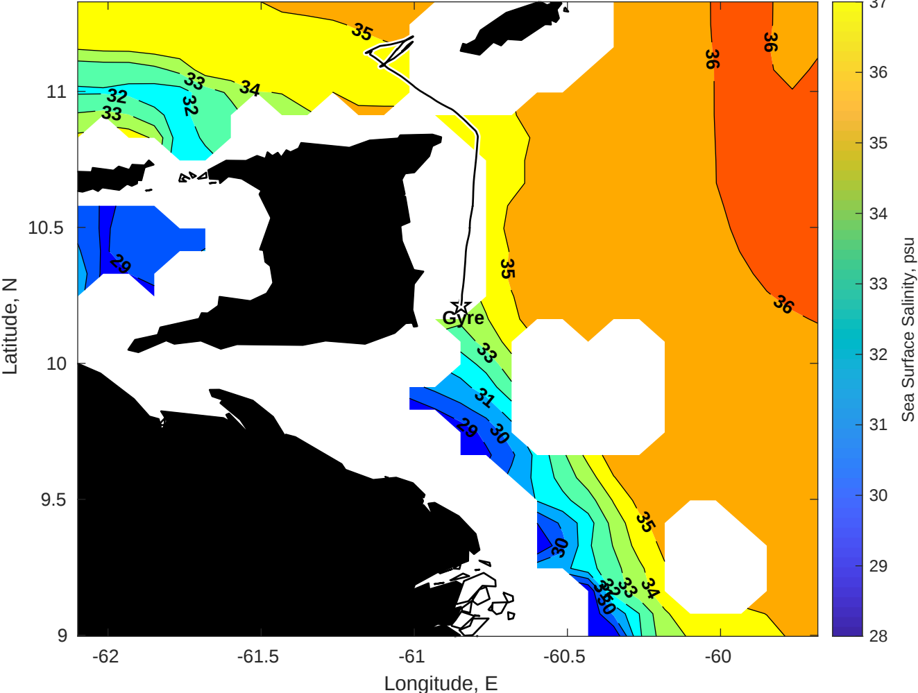
Surface Salinity for Gyre at 27-Dec-2025 00:00:00
