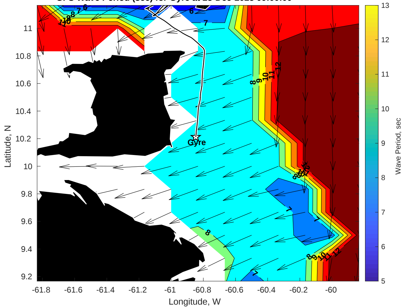
GFS Wave Period (sec) for Gyre at 28-Dec-2025 09:00:00
