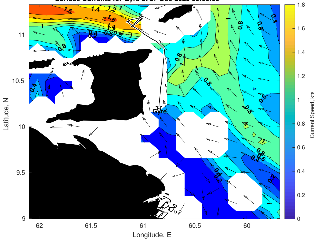
Surface Currents for Gyre at 27-Dec-2025 00:00:00
