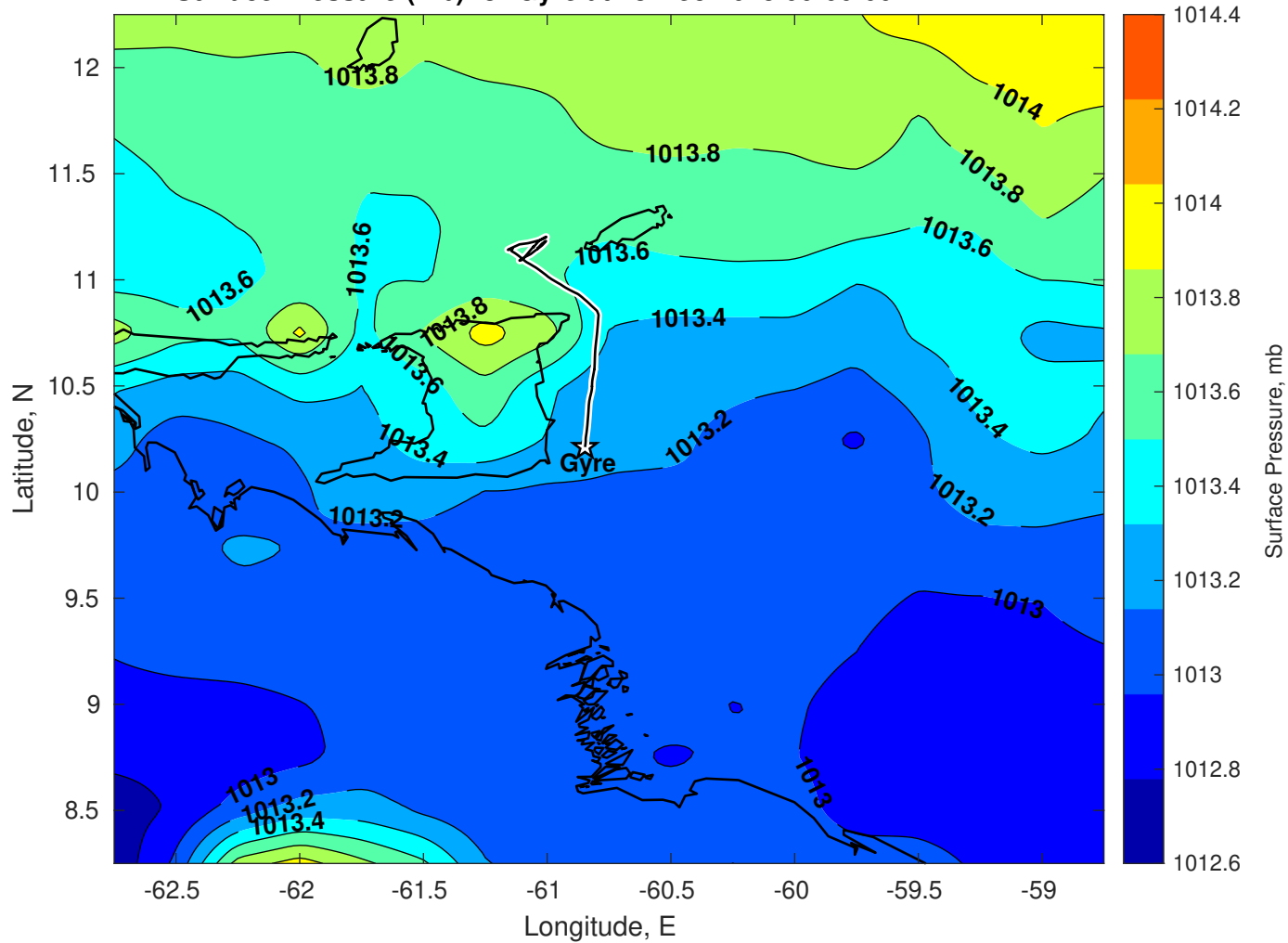
Surface Pressure (mb) for Gyre at 28-Dec-2025 00:00:00
