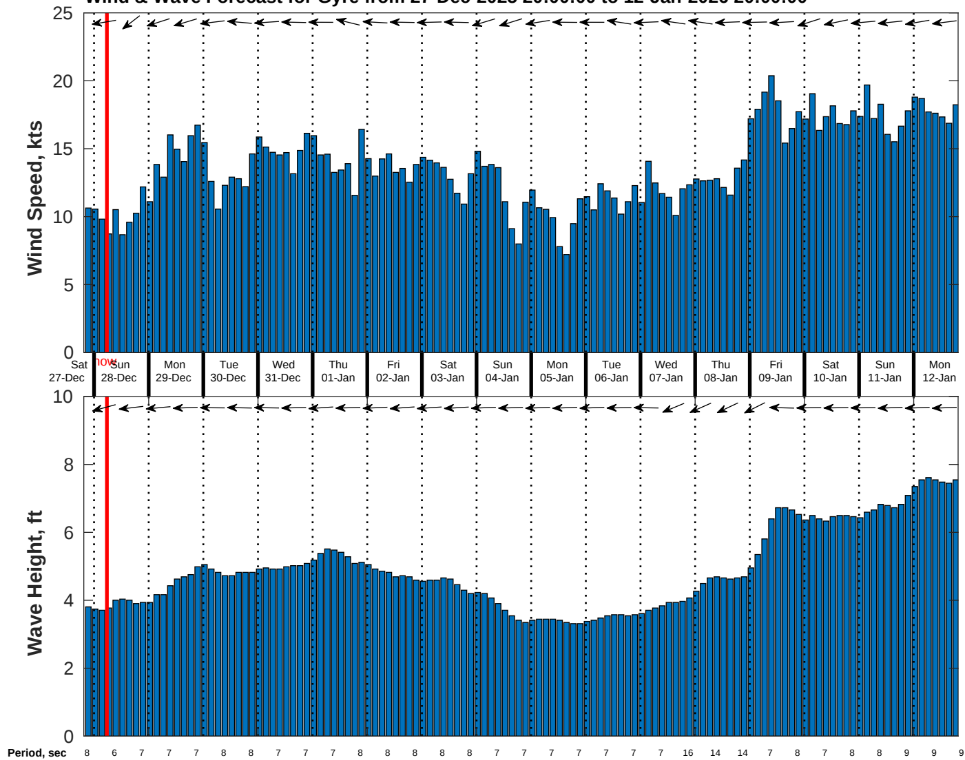
Wind & Wave Forecast for Gyre from 27-Dec-2025 20:00:00 to 12-Jan-2026 20:00:00
