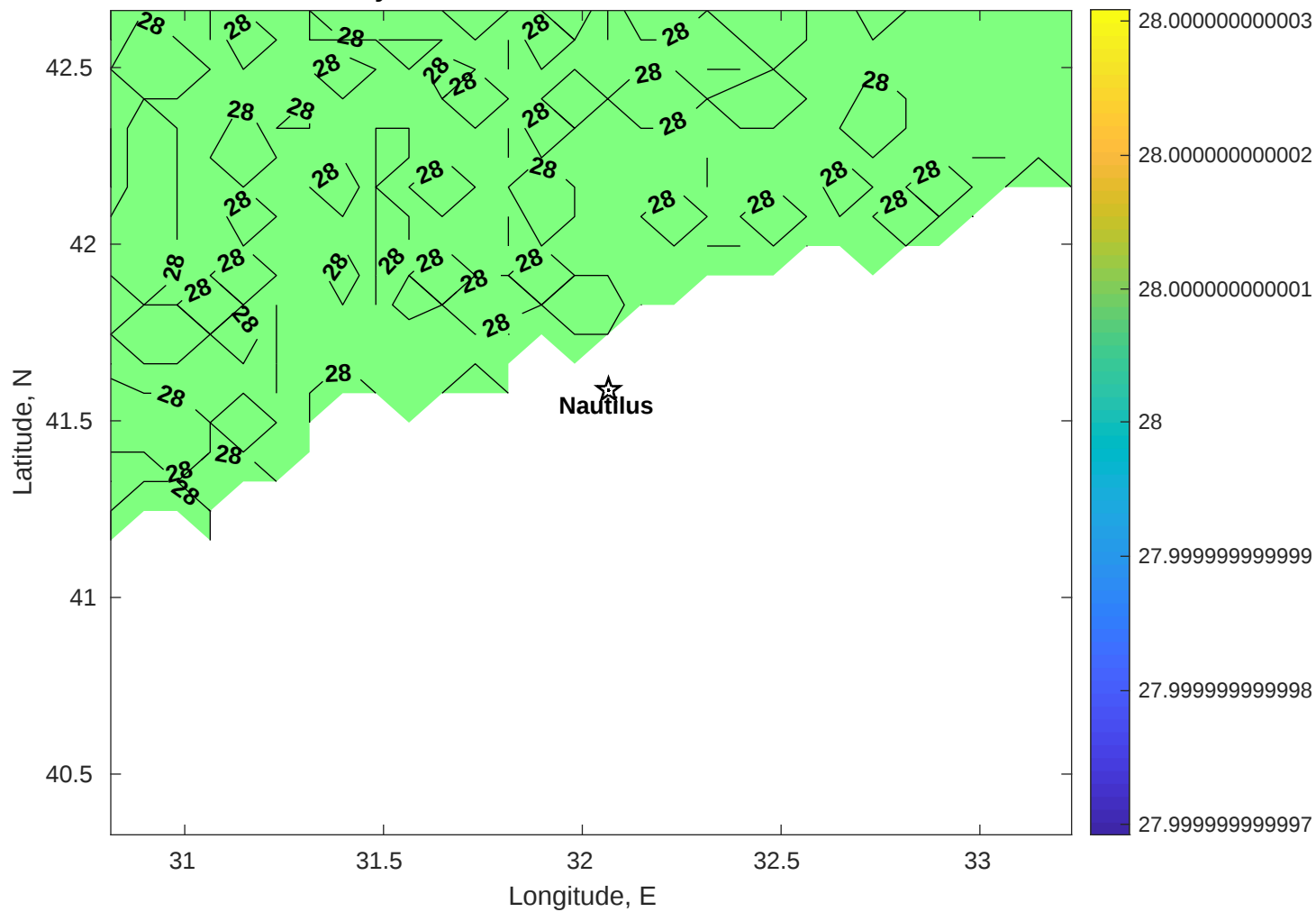
Surface Salinity for Nautilus at 27-Dec-2025 00:00:00
