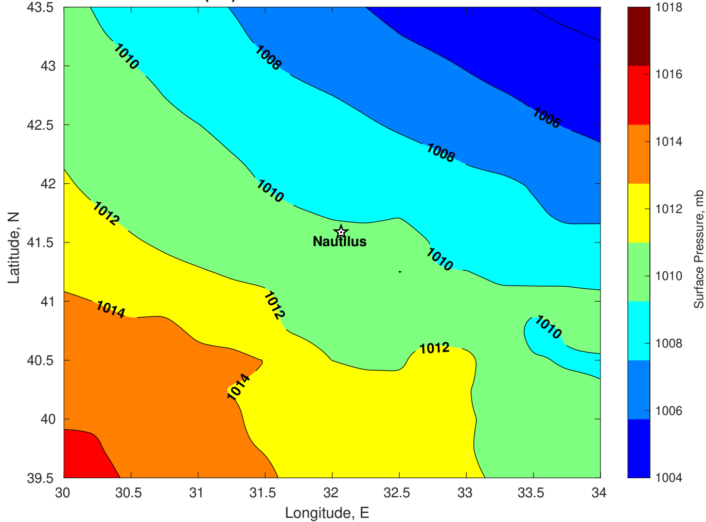
Surface Pressure (mb) for Nautilus at 29-Dec-2025 00:00:00
