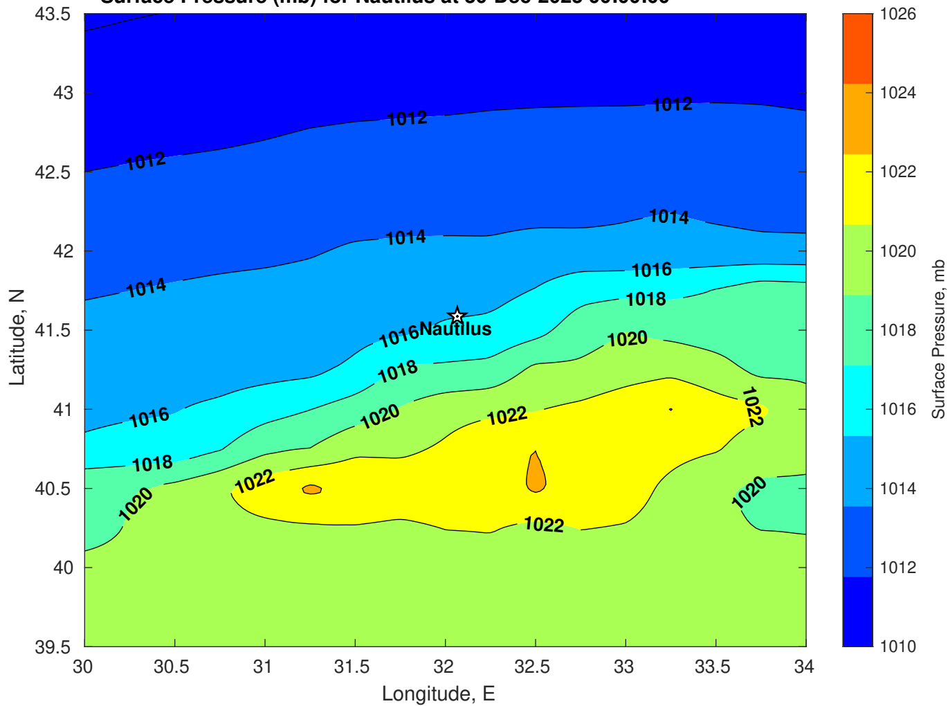
Surface Pressure (mb) for Nautilus at 30-Dec-2025 00:00:00
