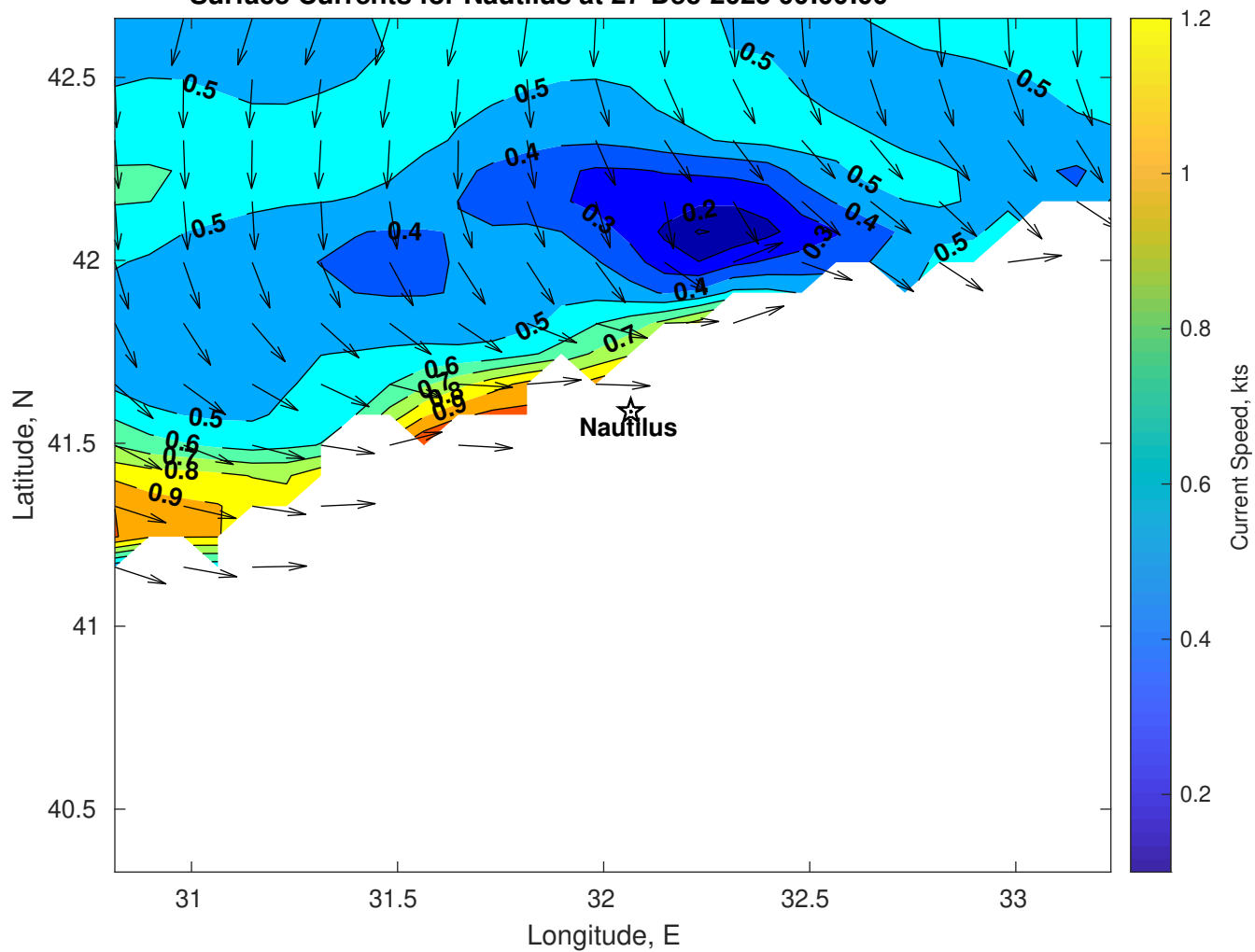
Surface Currents for Nautilus at 27-Dec-2025 00:00:00
