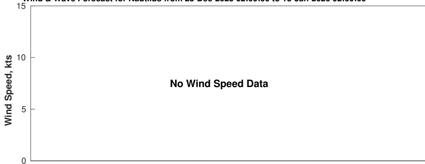
Wind & Wave Forecast for Nautilus from 28-Dec-2025 02:00:00 to 13-Jan-2026 02:00:00
