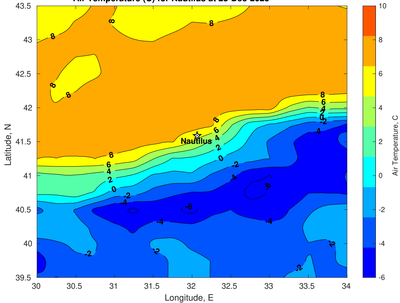
Air Temperature (C) for Nautilus at 28-Dec-2025
