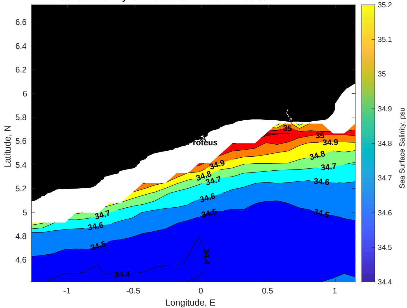
Surface Salinity for Proteus at 27-Dec-2025 00:00:00
