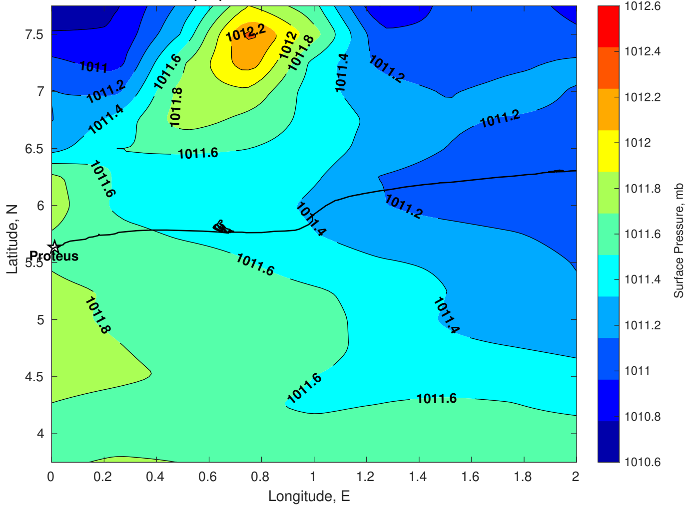
Surface Pressure (mb) for Proteus at 28-Dec-2025 00:00:00
