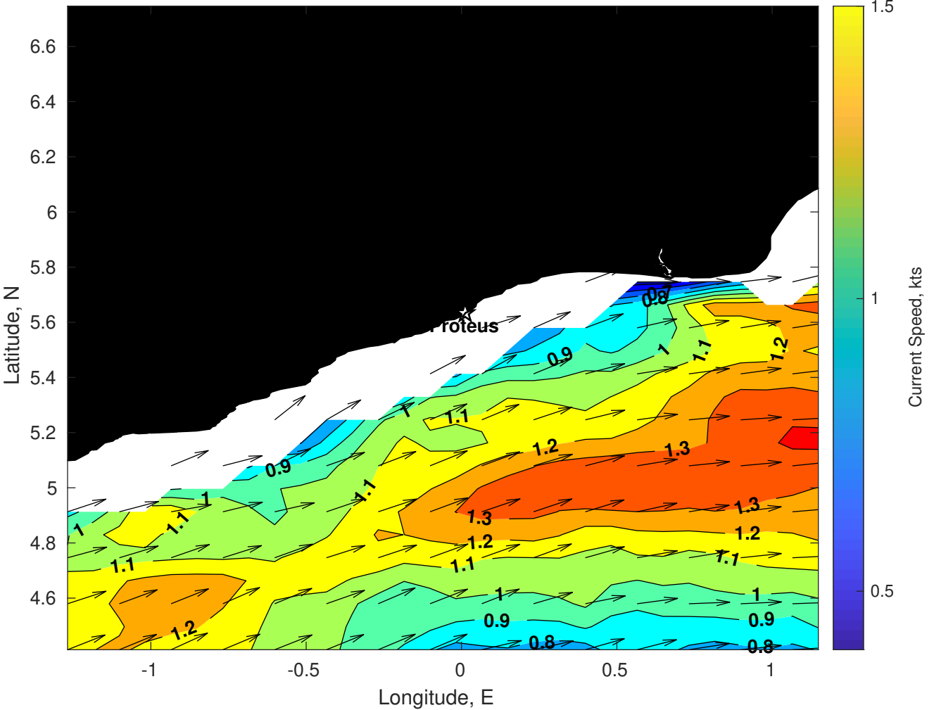
Surface Currents for Proteus at 27-Dec-2025 00:00:00
