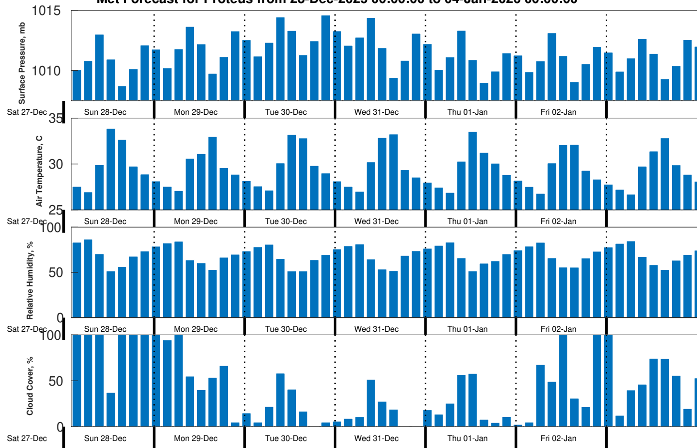
Met Forecast for Proteus from 28-Dec-2025 00:00:00 to 04-Jan-2026 00:00:00
