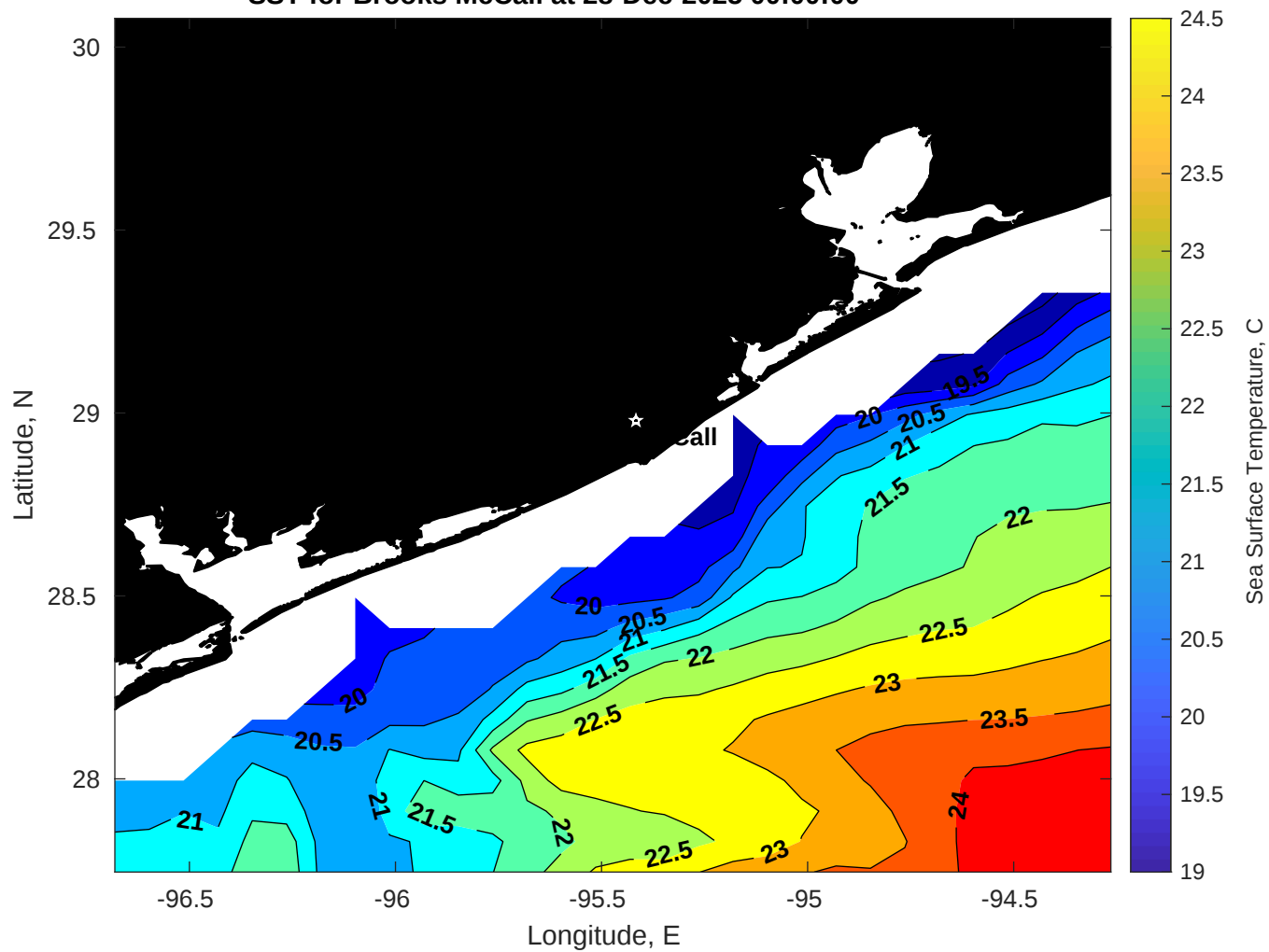
SST for Brooks McCall at 28-Dec-2025 00:00:00
