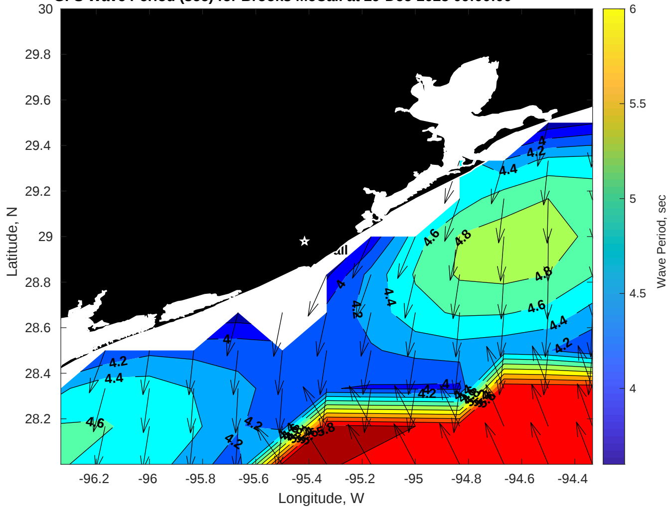
GFS Wave Period (sec) for Brooks McCall at 29-Dec-2025 09:00:00
