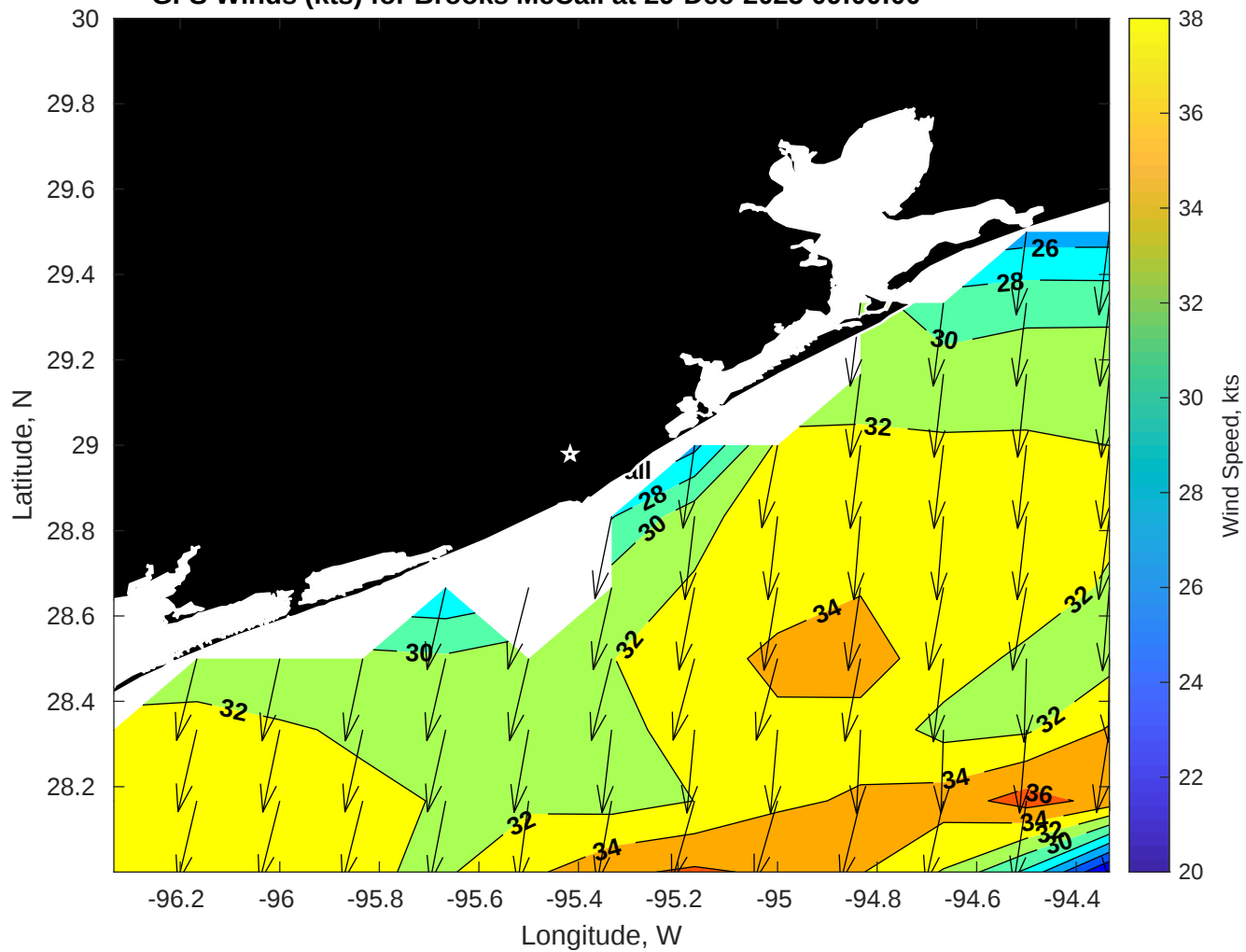
GFS Winds (kts) for Brooks McCall at 29-Dec-2025 09:00:00
