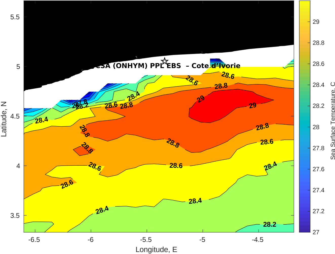
SST for CSA (ONHYM) PPL EBS - Cote d'Ivoire at 28-Dec-2025 00:00:00
