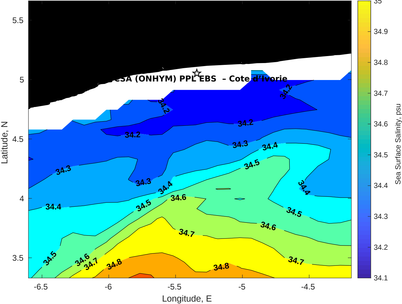
Surface Salinity for CSA (ONHYM) PPL EBS - Cote d'Ivoire at 28-Dec-2025 00:00:00
