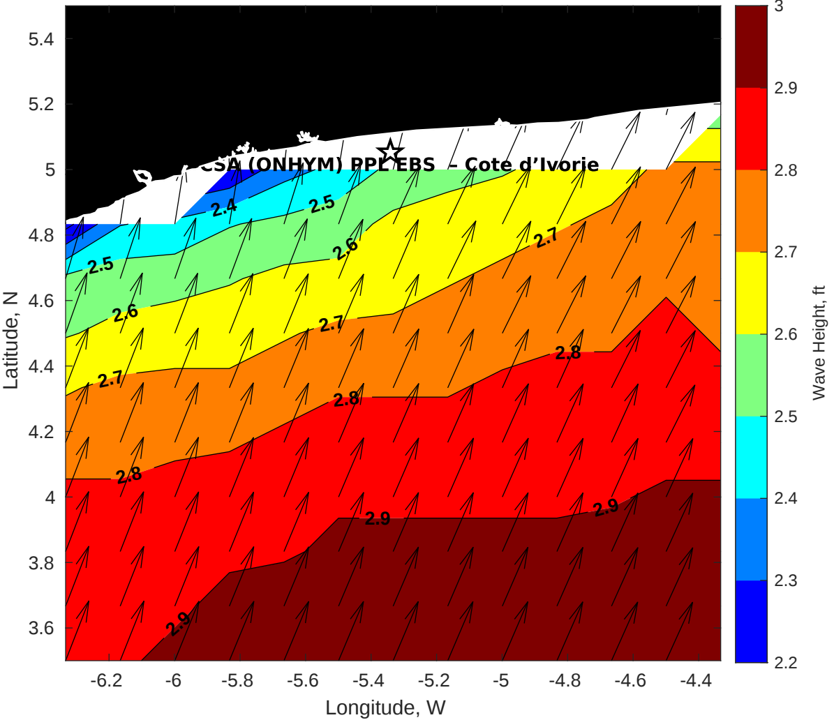
GFS Wave Height (ft) for CSA (ONHYM) PPL EBS - Cote d'Ivoire at 29-Dec-2025 09:00:00
