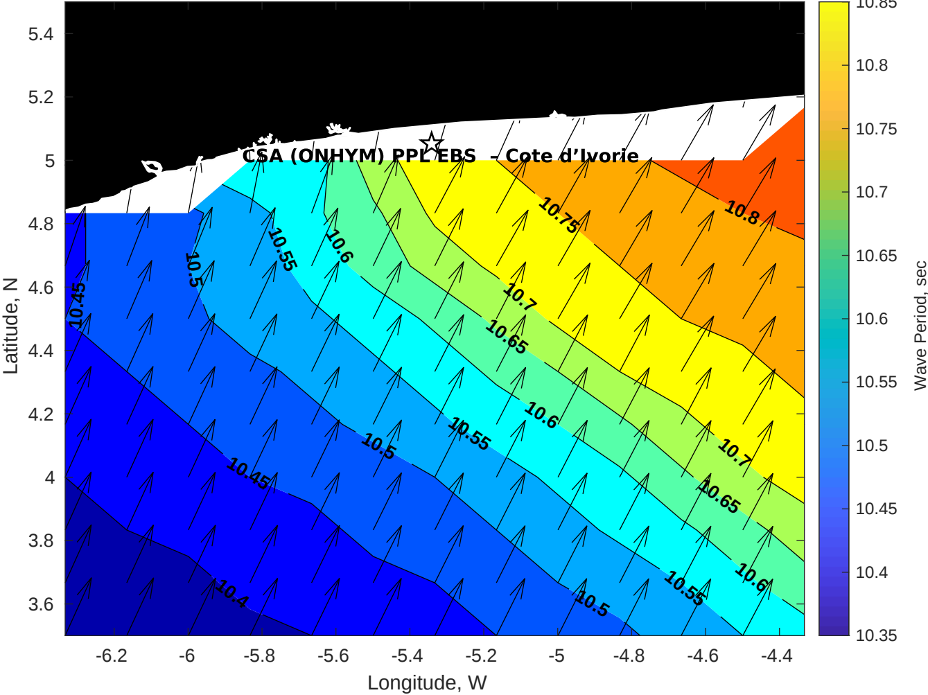
GFS Wave Period (sec) for CSA (ONHYM) PPL EBS - Cote d'Ivoire at 29-Dec-2025 09:00:00
