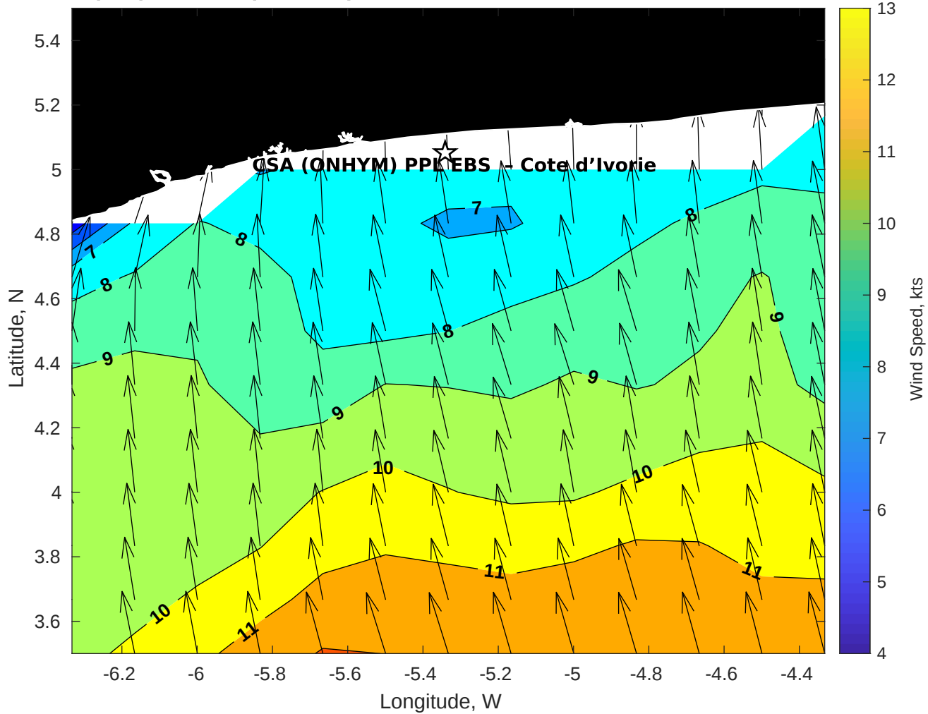
GFS Winds (kts) for CSA (ONHYM) PPL EBS - Cote d'Ivoire at 29-Dec-2025 09:00:00
