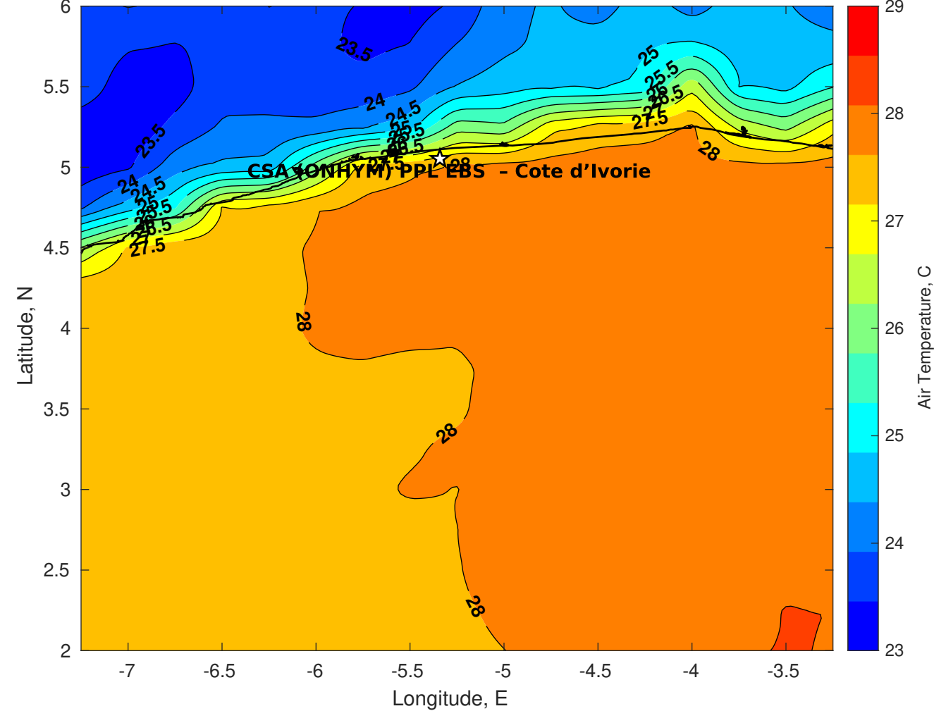
Air Temperature (C) for CSA (ONHYM) PPL EBS - Cote d'Ivoire at 29-Dec-2025
