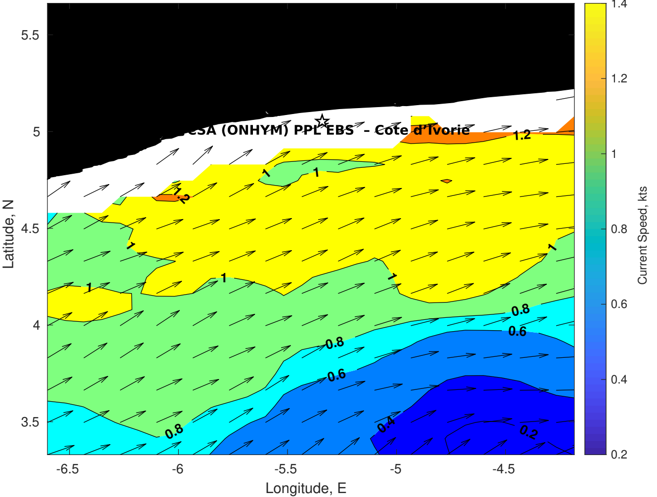
Surface Currents for CSA (ONHYM) PPL EBS - Cote d'Ivoire at 28-Dec-2025 00:00:00
