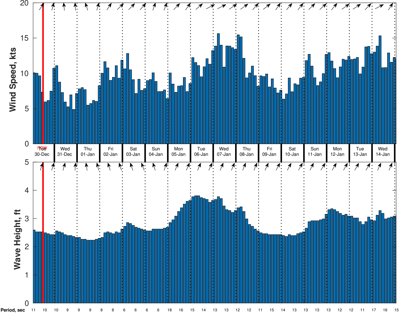
Wind & Wave Forecast for CSA (ONHYM) PPL EBS - Cote d'Ivoire from 29-Dec-2025 01:00:00 to 14-Jan-2026 01:00:00
