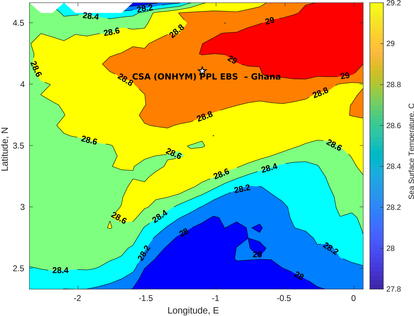
SST for CSA (ONHYM) PPL EBS - Ghana at 28-Dec-2025 00:00:00
