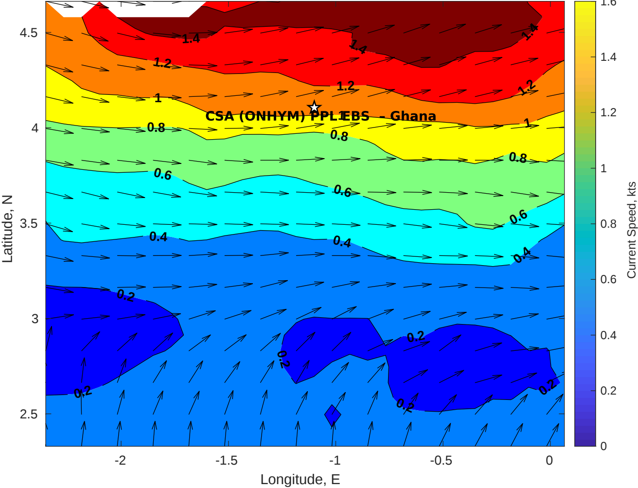
Surface Currents for CSA (ONHYM) PPL EBS - Ghana at 28-Dec-2025 00:00:00
