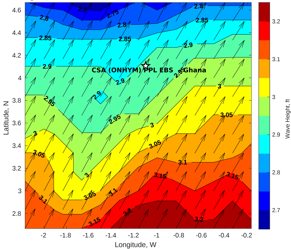
GFS Wave Height (ft) for CSA (ONHYM) PPL EBS - Ghana at 29-Dec-2025 09:00:00
