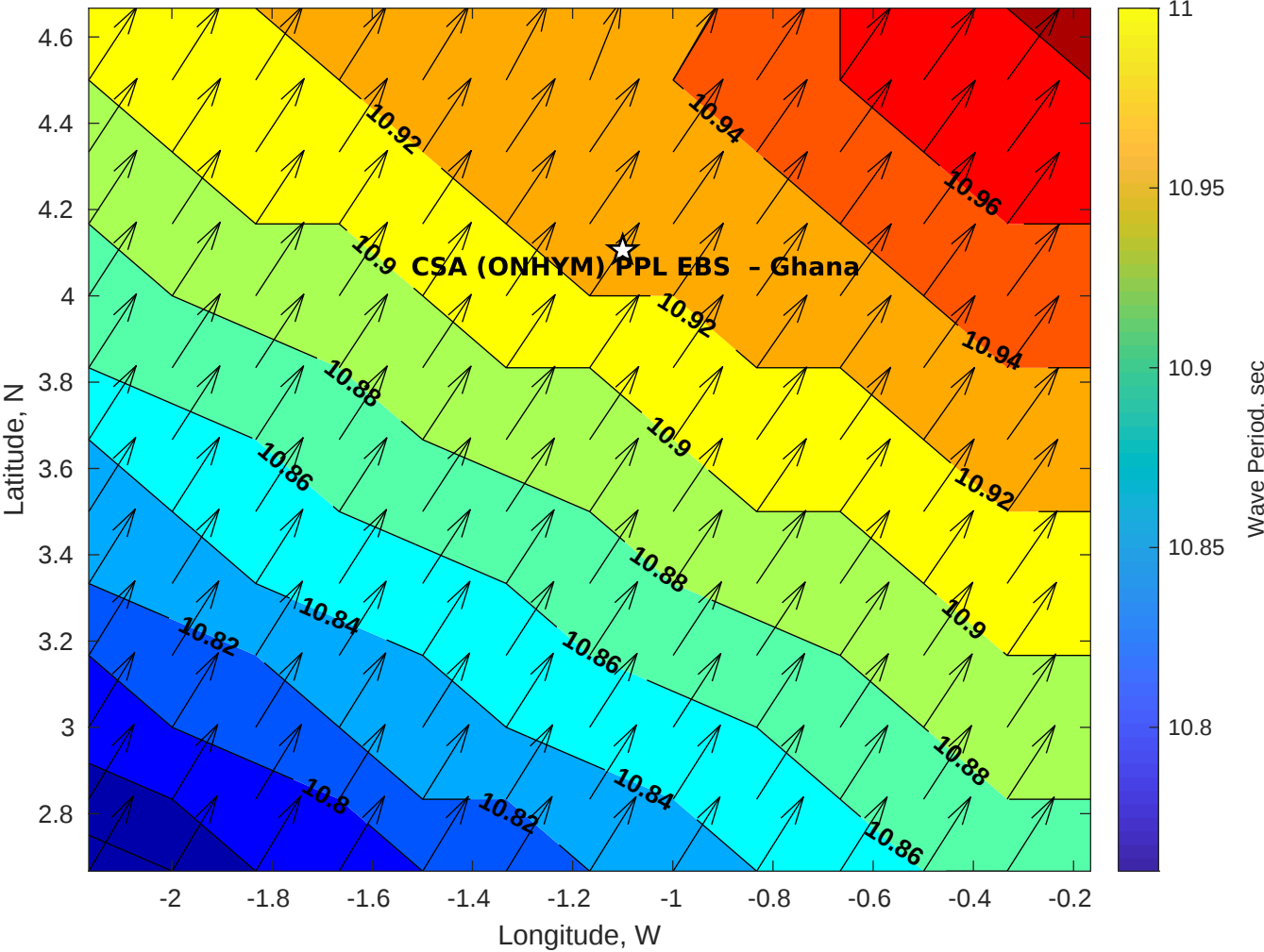
GFS Wave Period (sec) for CSA (ONHYM) PPL EBS - Ghana at 29-Dec-2025 09:00:00
