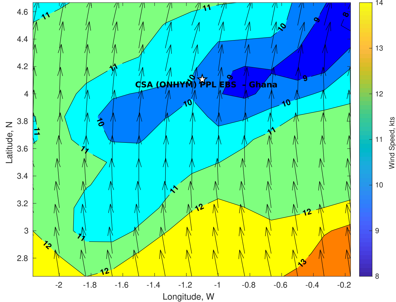
GFS Winds (kts) for CSA (ONHYM) PPL EBS - Ghana at 29-Dec-2025 09:00:00
