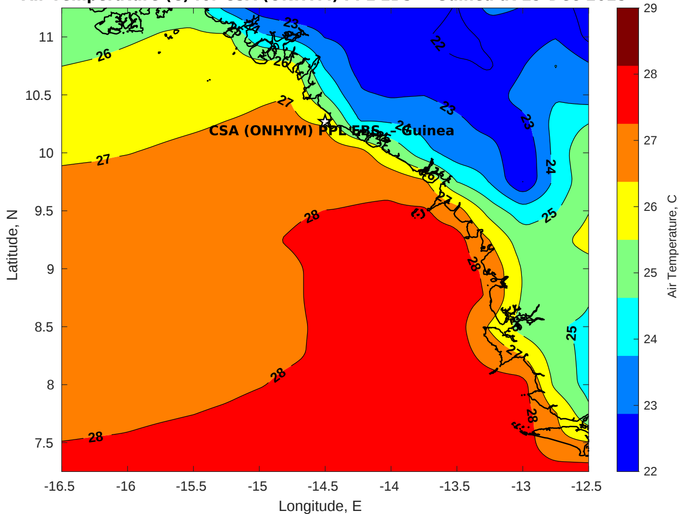
Air Temperature (C) for CSA (ONHYM) PPL EBS - Guinea at 29-Dec-2025
