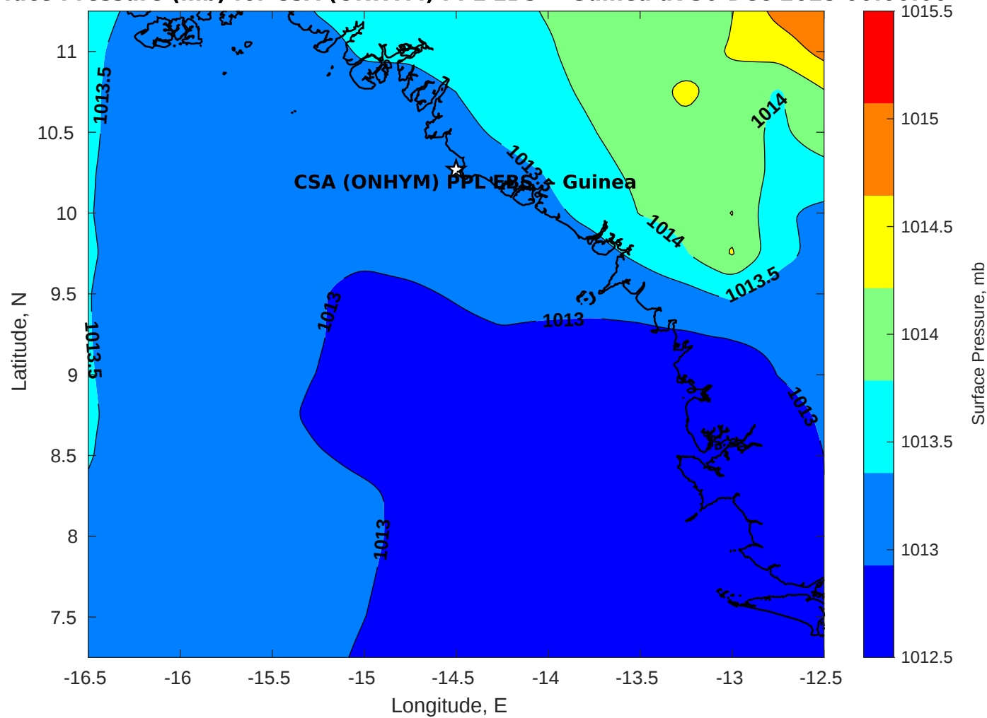
Surface Pressure (mb) for CSA (ONHYM) PPL EBS - Guinea at 30-Dec-2025 00:00:00
