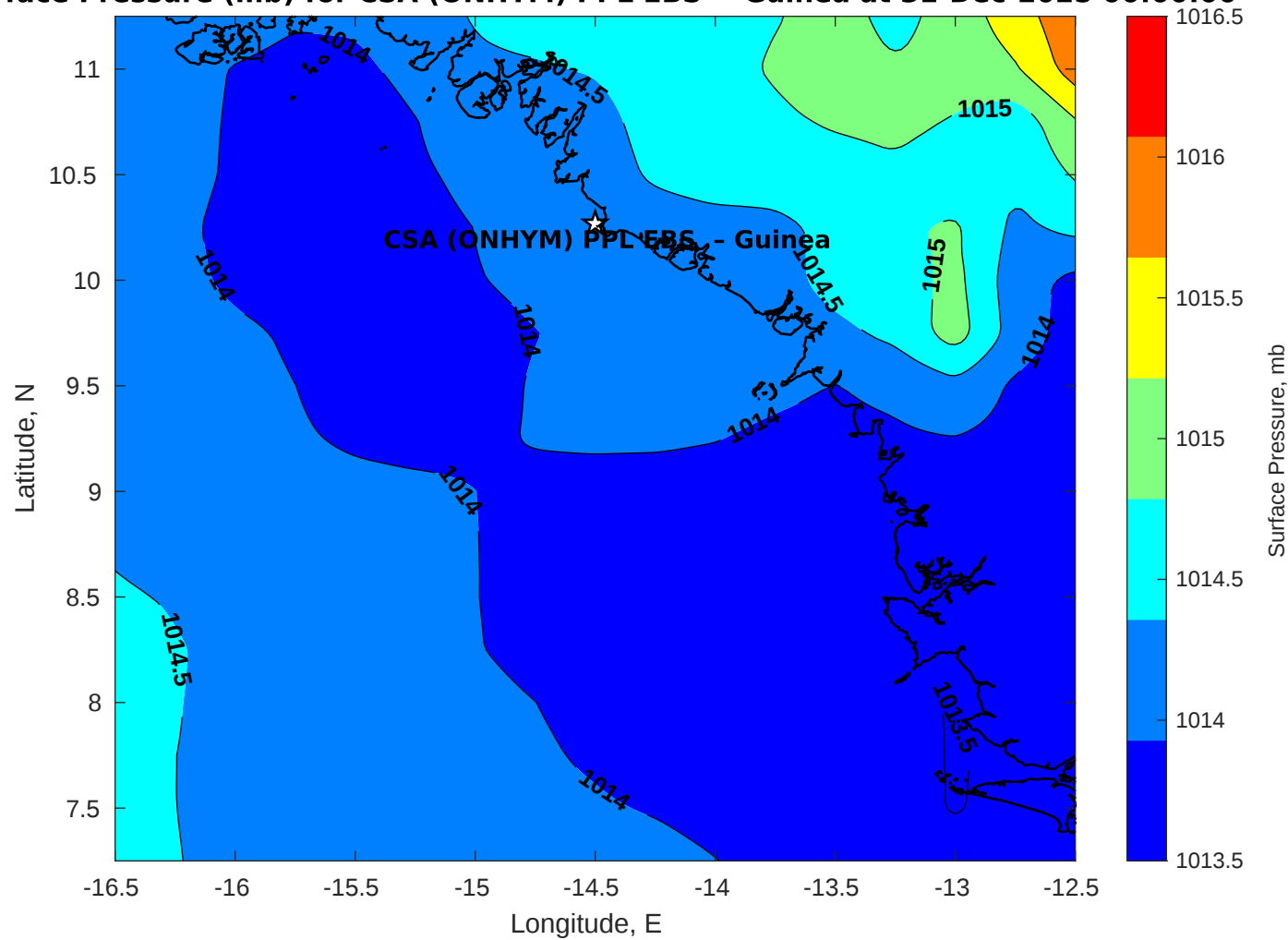
Surface Pressure (mb) for CSA (ONHYM) PPL EBS - Guinea at 31-Dec-2025 00:00:00
