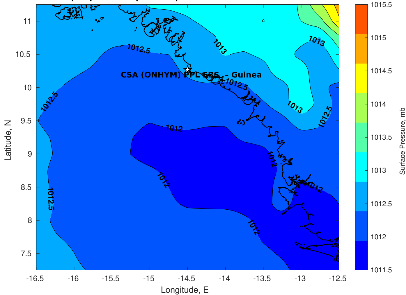
Surface Pressure (mb) for CSA (ONHYM) PPL EBS - Guinea at 29-Dec-2025 00:00:00
