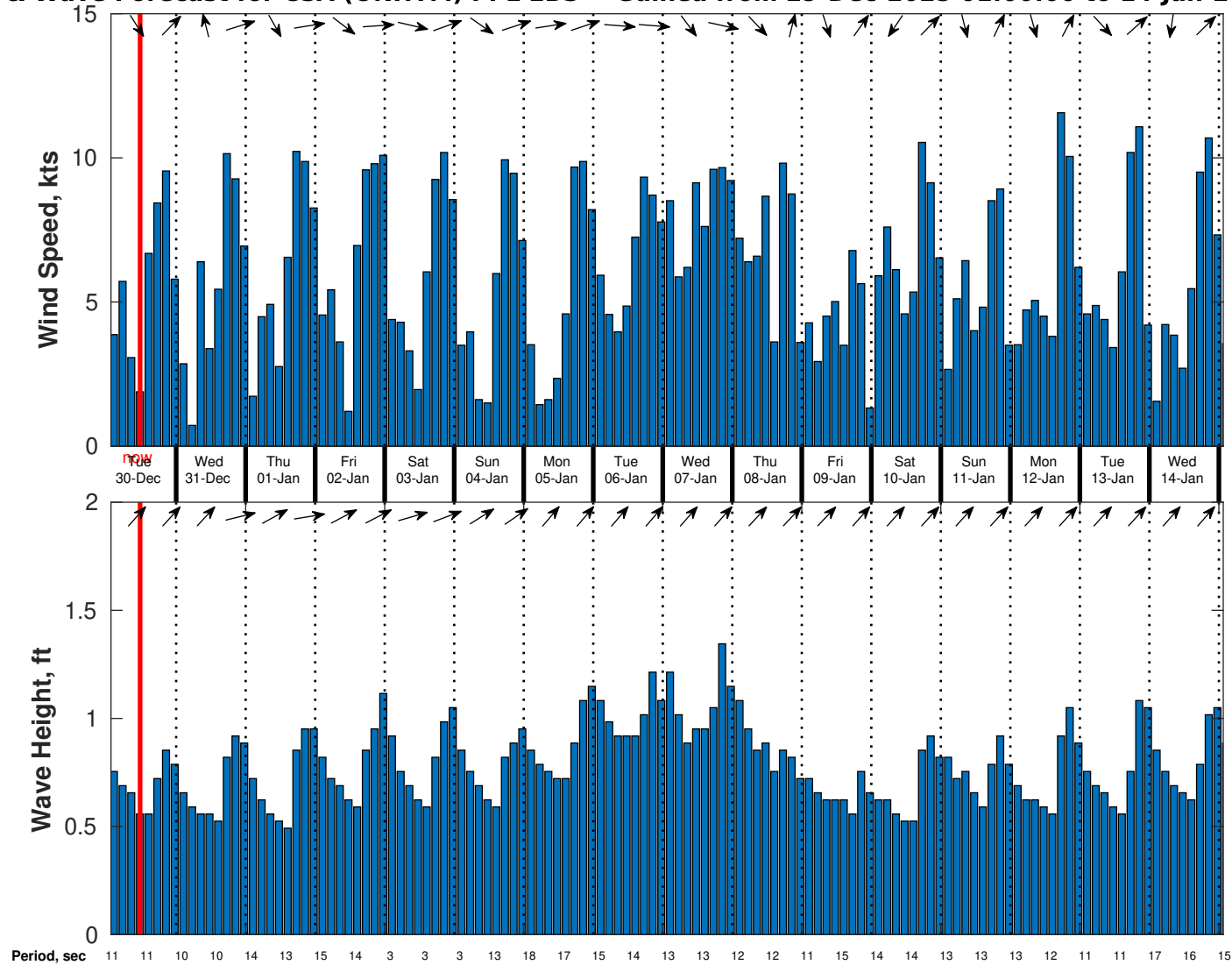
Wind & Wave Forecast for CSA (ONHYM) PPL EBS - Guinea from 29-Dec-2025 01:00:00 to 14-Jan-2026 01:00:00
