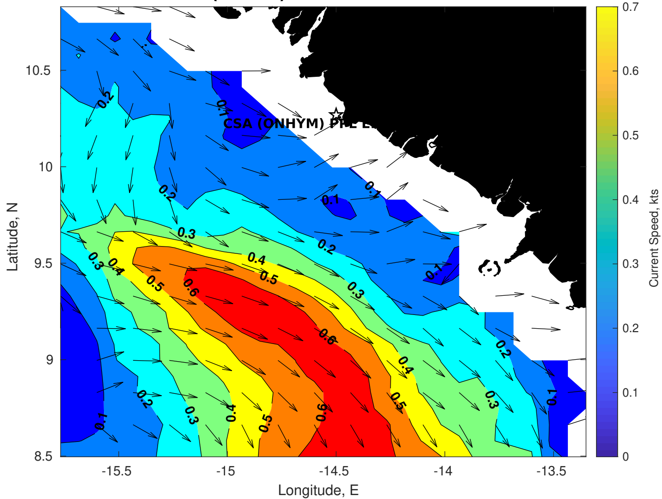
Surface Currents for CSA (ONHYM) PPL EBS - Guinea at 28-Dec-2025 00:00:00
