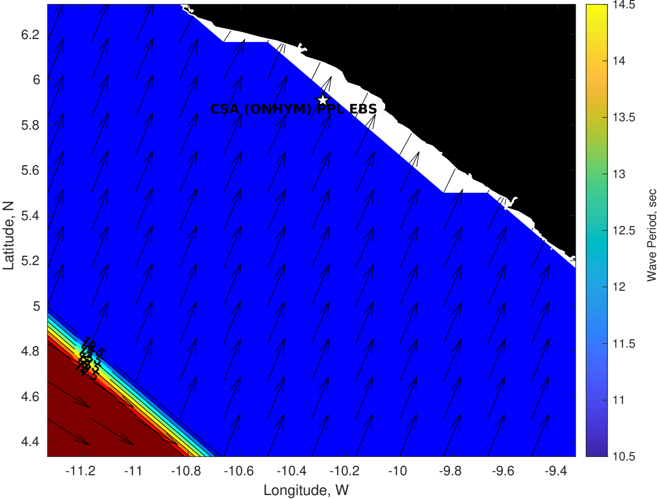
GFS Wave Period (sec) for CSA (ONHYM) PPL EBS - Liberia at 29-Dec-2025 09:00:00
