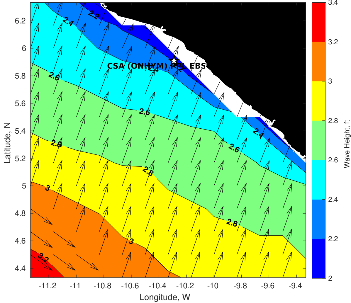
GFS Wave Height (ft) for CSA (ONHYM) PPL EBS - Liberia at 29-Dec-2025 09:00:00
