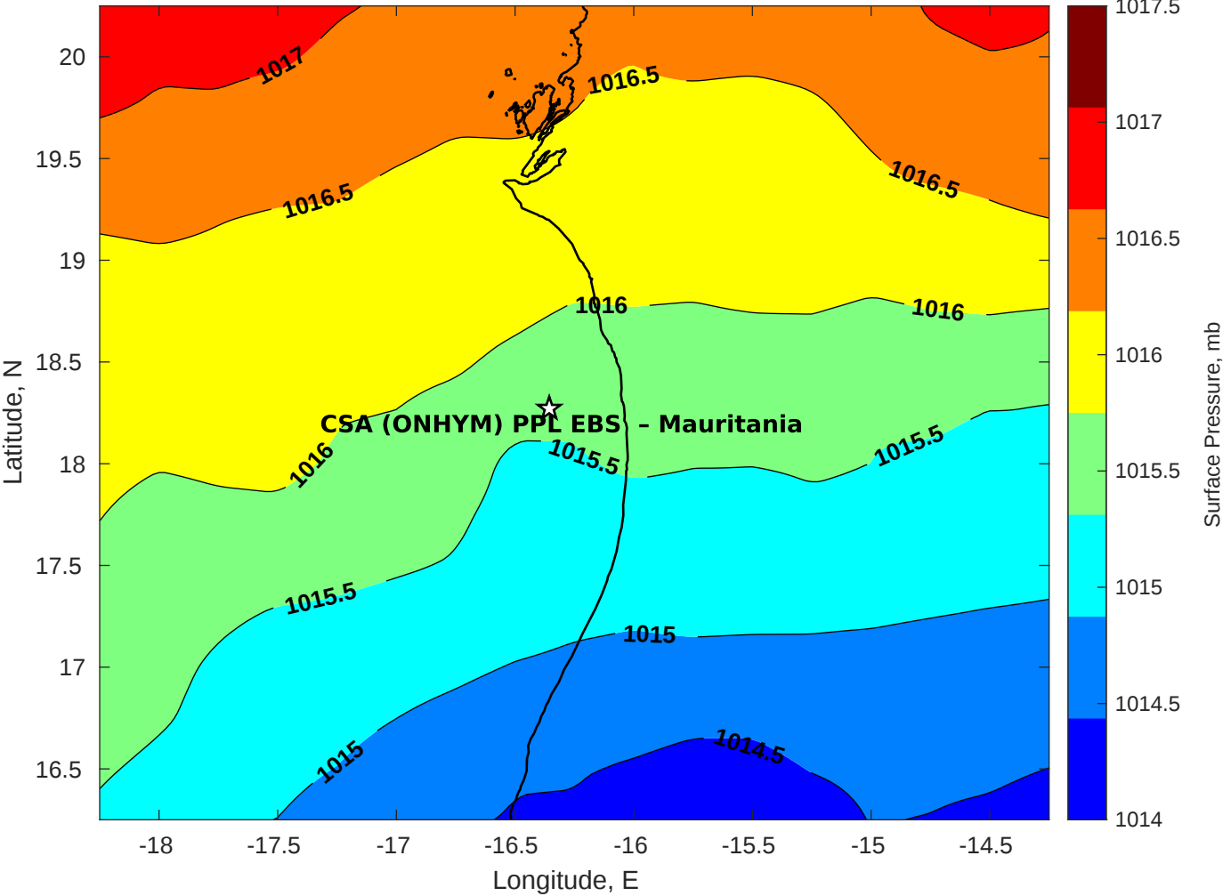
Surface Pressure (mb) for CSA (ONHYM) PPL EBS - Mauritania at 29-Dec-2025 00:00:00
