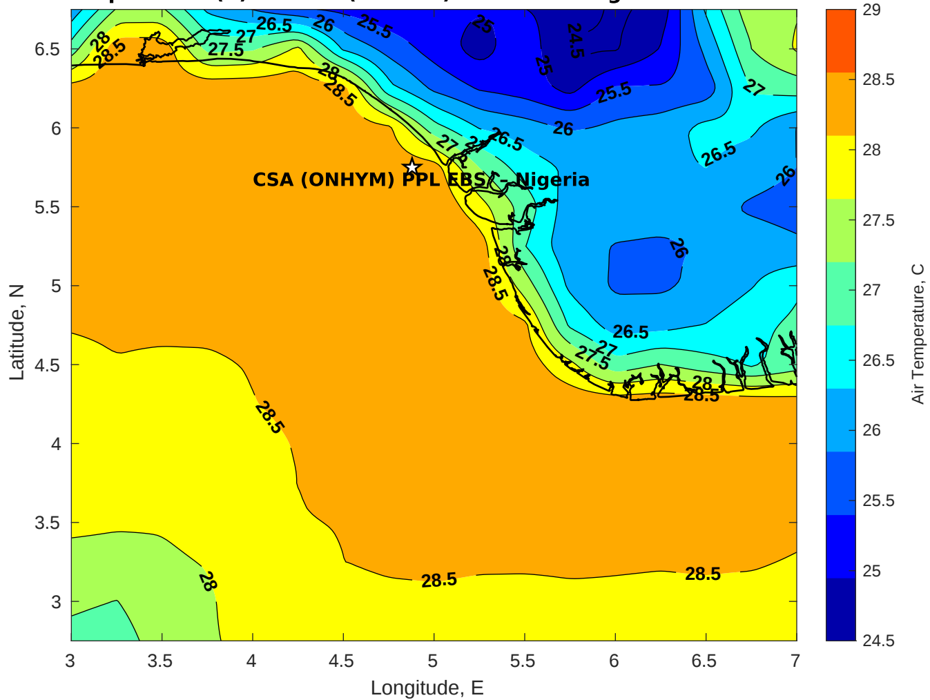
Air Temperature (C) for CSA (ONHYM) PPL EBS - Nigeria at 29-Dec-2025
