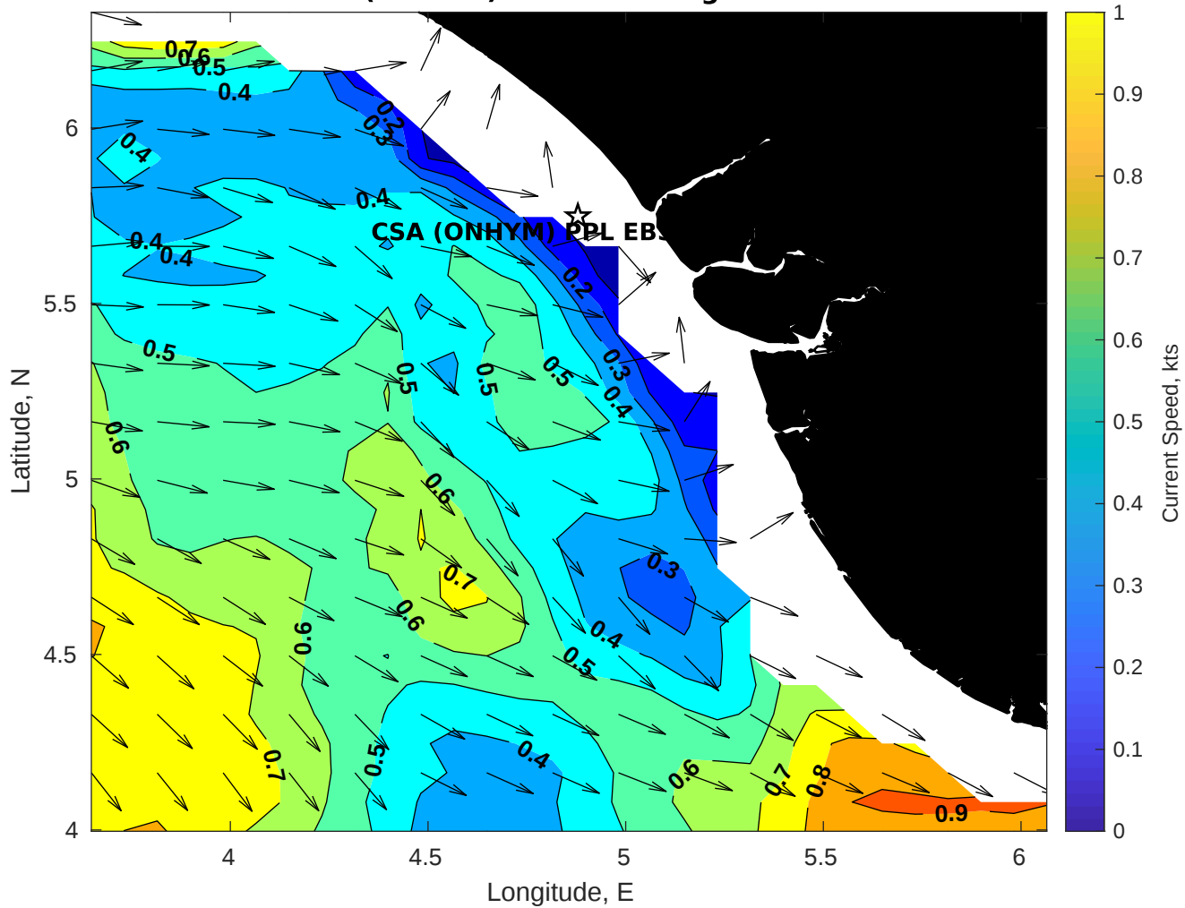
Surface Currents for CSA (ONHYM) PPL EBS - Nigeria at 28-Dec-2025 00:00:00
