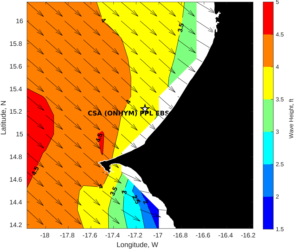
GFS Wave Height (ft) for CSA (ONHYM) PPL EBS - Senegal at 29-Dec-2025 09:00:00
