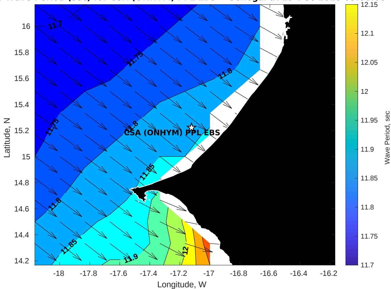
GFS Wave Period (sec) for CSA (ONHYM) PPL EBS - Senegal at 29-Dec-2025 09:00:00
